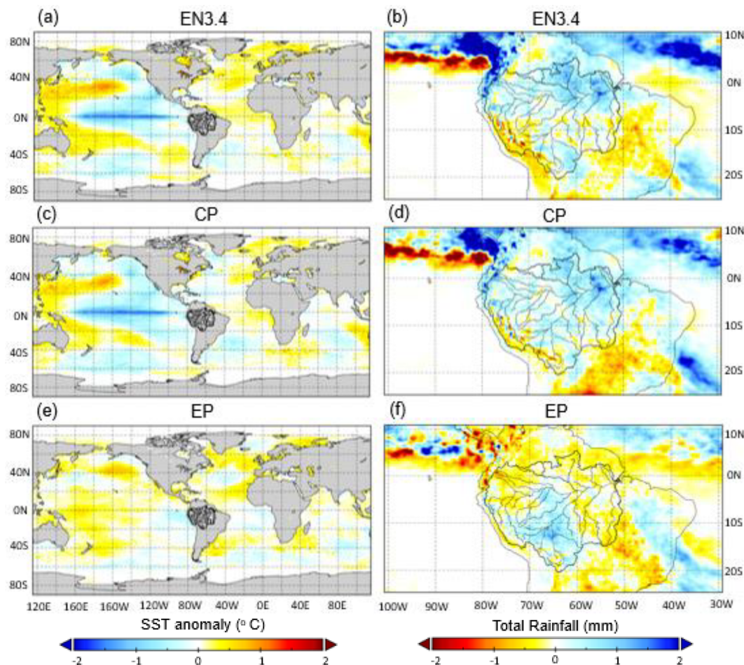
Figure 12. Composite analysis of the difference between the preceding OND average SST ( ^{\circ}\text{C} ) ( a , c , e ) and total rainfall (mm) ( b , d , f ) for the average of the 12 negative years and the average of the 12 neutral years. Panels ( a , b ): EN3.4 index; panels ( c , d ): CP index; and panels ( e , f ): EP index. A list of the negative and neutral years for each index can be found in Tables S2, S4 and S5 in the Supplement.
