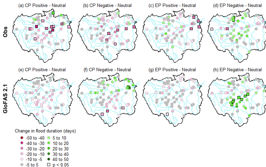
Figure 9. Changes in flood duration (i.e. mean number of days river flows exceed the 95th percentile of each station or grid point climatology) for different phases of the CP and EP indices. (a, c, e, g) Positive with respect to neutral years. (b, d, f, h) Negative with respect to neutral years. Panels (a–d) represent changes for observations and panels (e–h) show changes for GloFAS 2.1 streamflow reanalysis data. Pink (green) points represent decreases (increases) in the number of days spent above the 95th percentile compared to neutral conditions. Significant results at the 95 % confidence level are denoted using a square (i.e. p < 0.05 ).
