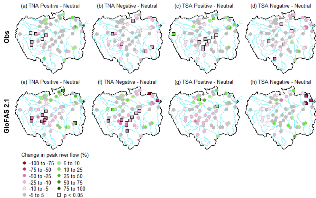
Figure 4. Percentage change of observed and simulated mean annual peak river flows between different phases of tropical Atlantic indices. (a, c, e, g) Positive with respect to neutral years. (b, d, f, h) Negative with respect to neutral years. Panels (a–d) represent changes for observations and panels (e–h) show changes for GloFAS 2.1 streamflow reanalysis data. Pink (green) points represent where the average annual peak flow decreases (increases). Significant results at the 95 % confidence level are denoted using a square (i.e. p < 0.05 ).
