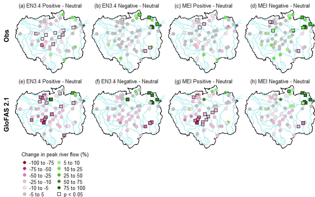
Figure 2. Percentage change of observed and simulated mean annual peak river flows between different phases of the EN3.4 and MEI indices. (a, c, e, g) Positive with respect to neutral years. (b, d, f, h) Negative with respect to neutral years. Panels (a–d) represent changes for observations and panels (e–h) show changes for GloFAS 2.1 streamflow reanalysis data. Pink (green) points represent where the average annual peak flow decreases (increases). Significant results at the 95 % confidence level are denoted using a square (i.e. p < 0.05 ).
