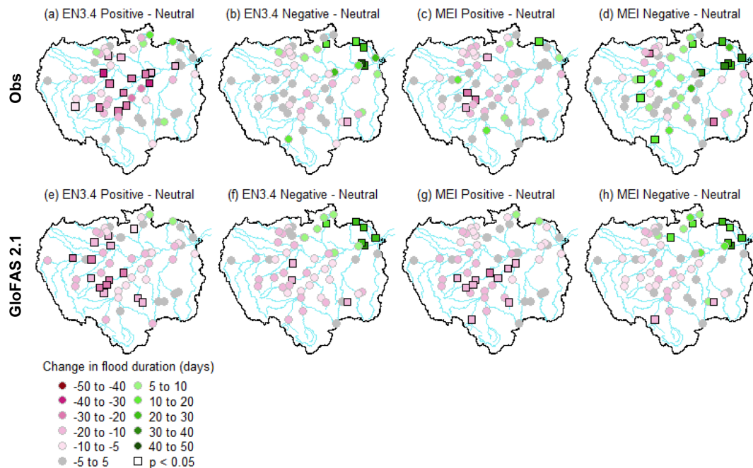
Figure 8. Changes in flood duration (i.e. mean number of days river flows exceed the 95th percentile of each station or grid point climatology) for different phases of the EN3.4 and MEI indices. (a, c, e, g) Positive with respect to neutral years. (b, d, f, h) Negative with respect to neutral years. Panels (a–d) represent changes for observations and panels (e–h) show changes for GloFAS 2.1 streamflow reanalysis data. Pink (green) points represent decreases (increases) in the number of days spent above the 95th percentile compared to neutral conditions. Significant results at the 95 % confidence level are denoted using a square (i.e. p < 0.05 ).
