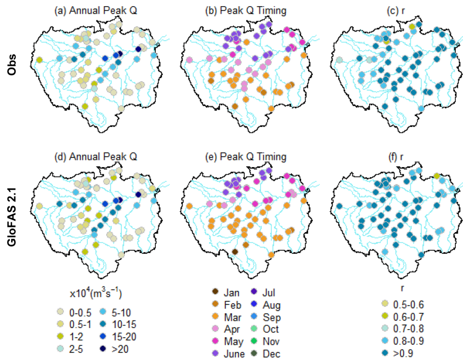
Figure 1. 36-year climatology of observed (a–c) and GloFAS 2.1 streamflow reanalysis (d–f) datasets (1979–2015). (a, d) Mean annual maximum river flows. (b, e) Average timing of peak flow occurrences. (c, f) Interannual variability of peak flow timing (i.e. the consistency of when rivers reach their peaks). Values closer to 1 mean that rivers reach their peak at a similar time each hydrological year, whereas values closer to zero reflect a highly variable regime where flood peaks are spread through the year).
