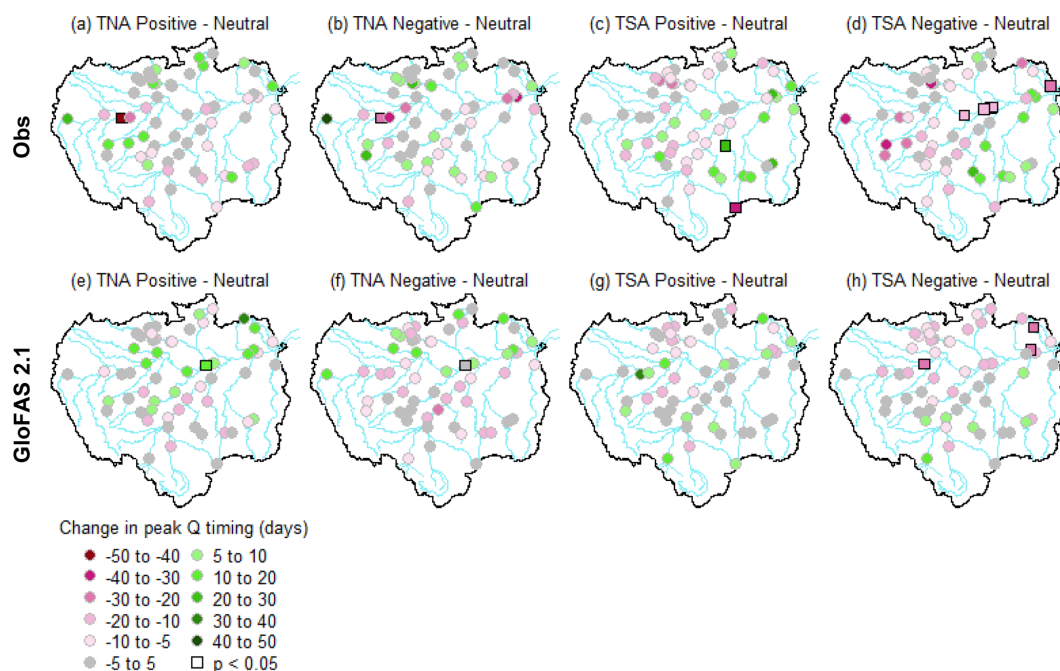
Figure 7. Average change in the timing of observed and simulated annual peak river flows between different phases of tropical Atlantic indices. (a, c, e, g) Positive with respect to neutral years. (b, d, f, h) Negative with respect to neutral years. Panels (a–d) represent changes for observations and panels (e–h) show changes for GloFAS 2.1 streamflow reanalysis data. Pink (green) points represent where flood peaks occur earlier (later) compared to neutral conditions. Significant results at the 95 % confidence level are denoted using a square (i.e. p < 0.05 ).
