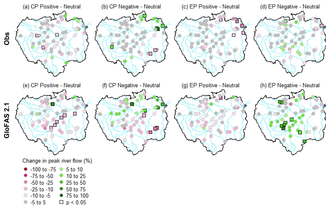
Figure 3. Percentage change of observed and simulated mean annual peak river flows between different phases of the CP and EP indices. (a, c, e, g) Positive with respect to neutral years. (b, d, f, h) Negative with respect to neutral years. Panels (a–d) represent changes for observations and panels (e–h) show changes for GloFAS 2.1 streamflow reanalysis data. Pink (green) points represent where the average annual peak flow decreases (increases). Significant results at the 95 % confidence level are denoted using a square (i.e. p < 0.05 ).
