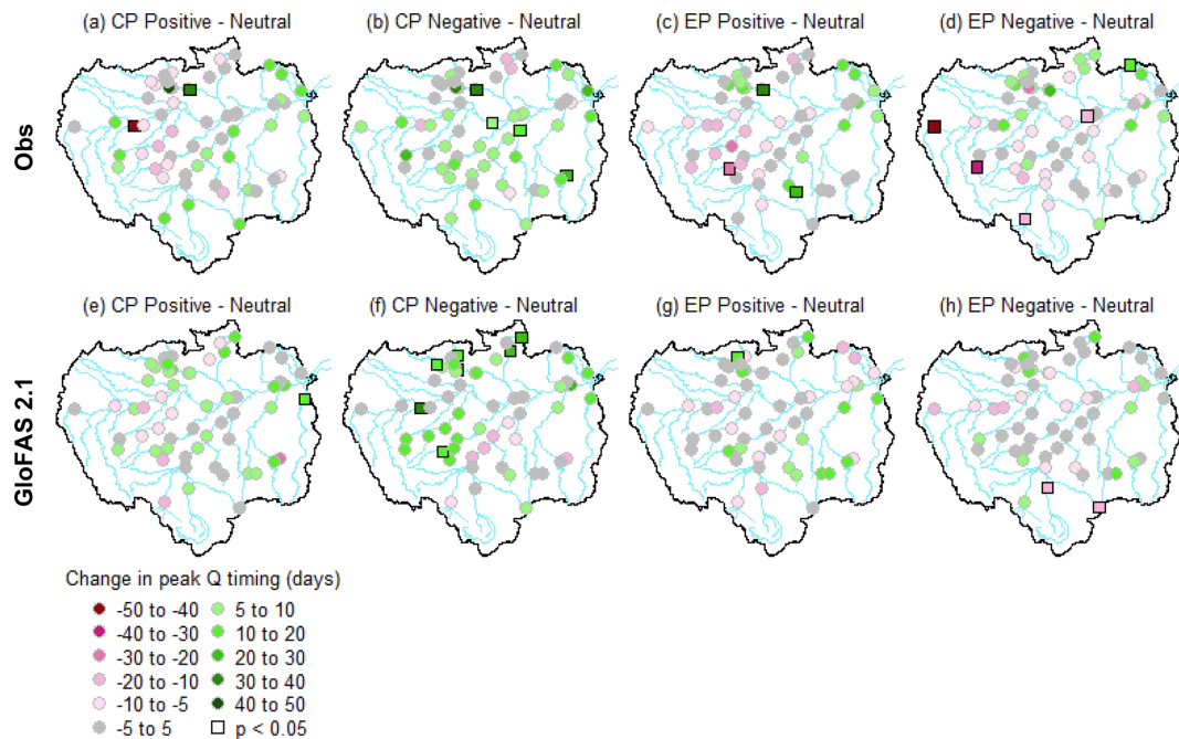
Figure 6. Average change in the timing of observed and simulated annual peak river flows between different phases of the CP and EP indices. (a, c, e, g) Positive with respect to neutral years. (b, d, f, h) Negative with respect to neutral years. Panels (a–d) represent changes for observations and panels (e–h) show changes for GloFAS 2.1 streamflow reanalysis data. Pink (green) points represent where flood peaks occur earlier (later) compared to neutral conditions. Significant results at the 95 % confidence level are denoted using a square (i.e. p < 0.05 ).
