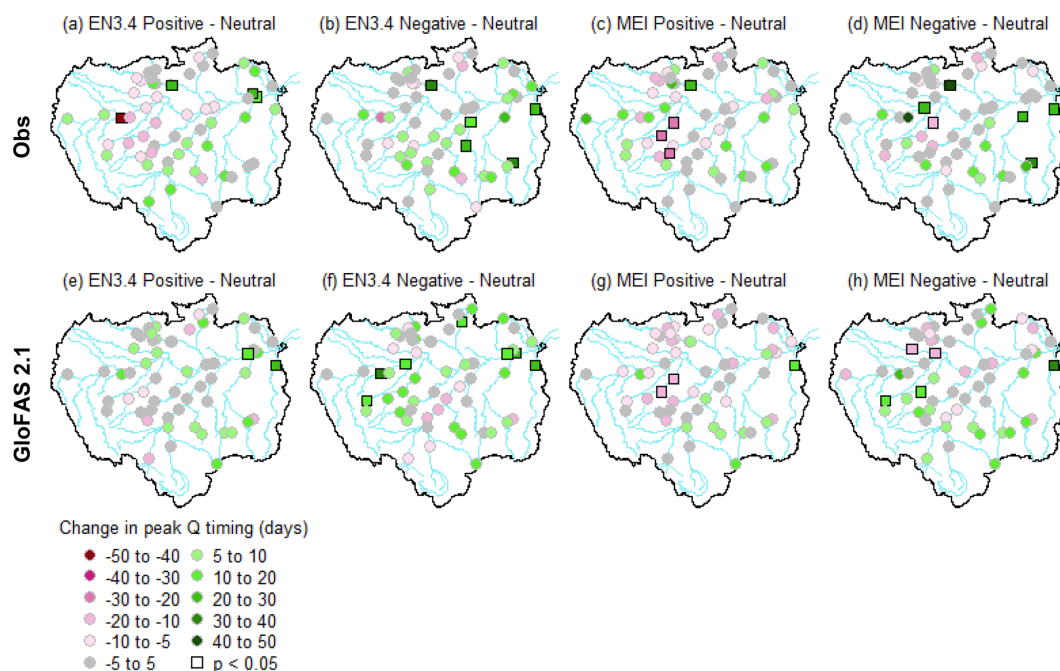
Figure 5. Average change in the timing of observed and simulated annual peak river flows between different phases of the EN3.4 and MEI indices. (a, c, e, g) Positive with respect to neutral years. (b, d, f, h) Negative with respect to neutral years. Panels (a–d) represent changes for observations and panels (e–h) show changes for GloFAS 2.1 streamflow reanalysis data. Pink (green) points represent where flood peaks occur earlier (later) compared to neutral conditions. Significant results at the 95 % confidence level are denoted using a square (i.e. p < 0.05 ).
