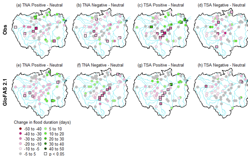
Figure 10. Changes in flood duration (i.e. mean number of days river flows exceed the 95th percentile of each station or grid point climatology) for different phases of tropical Atlantic indices. (a, c, e, g) Positive with respect to neutral years. (b, d, f, h) Negative with respect to neutral years. Panels (a–d) represent changes for observations and panels (e–h) show changes for GloFAS 2.1 streamflow reanalysis data. Pink (green) points represent decreases (increases) in the number of days spent above the 95th percentile compared to neutral conditions. Significant results at the 95 % confidence levels are denoted using a square (i.e. p < 0.05 ).
