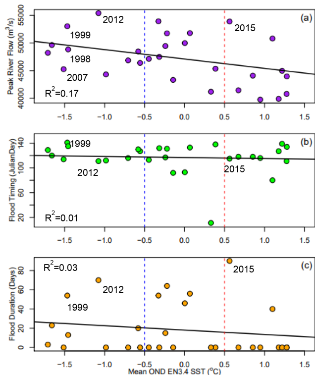
Figure 11. Scatterplot of the mean OND SST anomaly in the EN3.4 region vs. (a) the annual river flow magnitude, (b) peak flow timing and (c) flood duration (i.e. days over the 95th percentile of flow) for the Tamshiyacu (2) gauging station for the period 1986–2015. Straight black lines represent the regression line, with the R^2 value provided for each. Major flood events are highlighted by the respective year.
