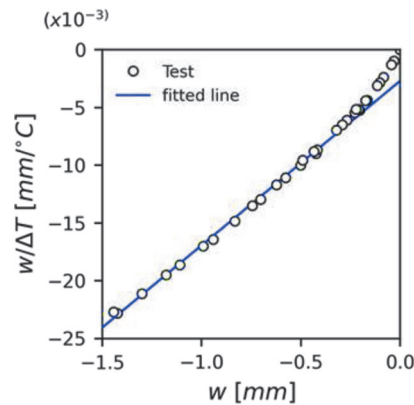
Fig. 7. Southwell plot for [30/-30/5/-5]_s plate.
