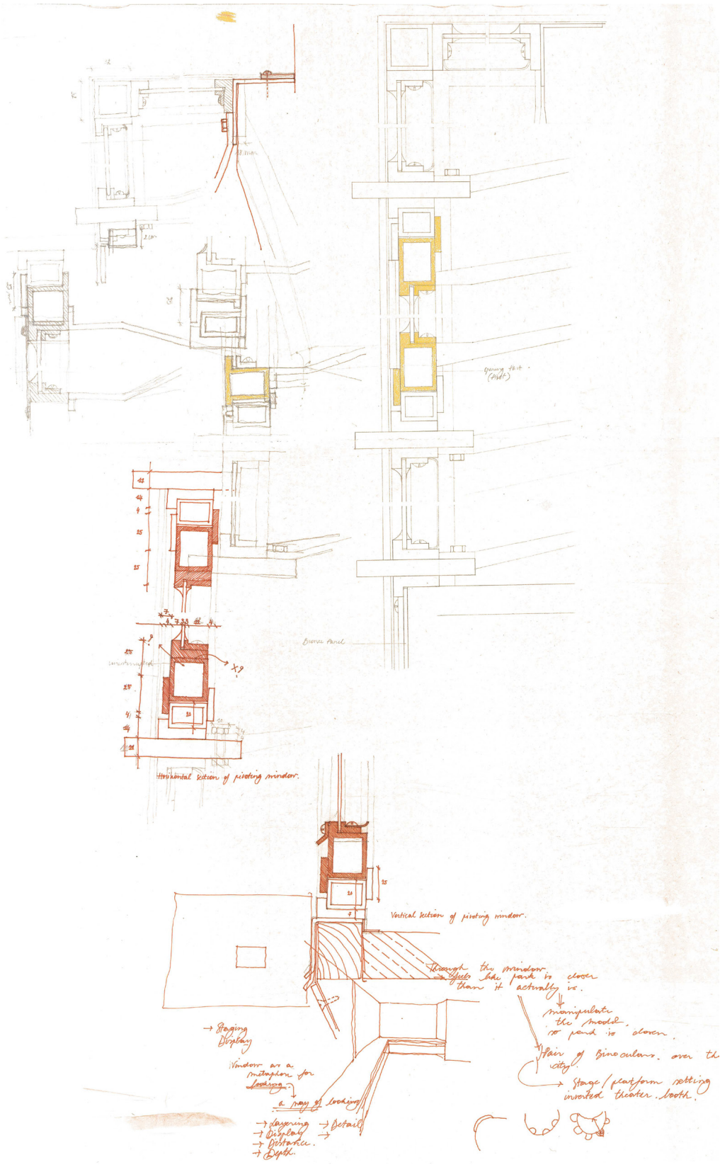
Fig. 1 Louise De Brabander, Revision Drawing of the Windowframes of a Corner Window at De Grote Post in Ostend, Ghent, 2020.
