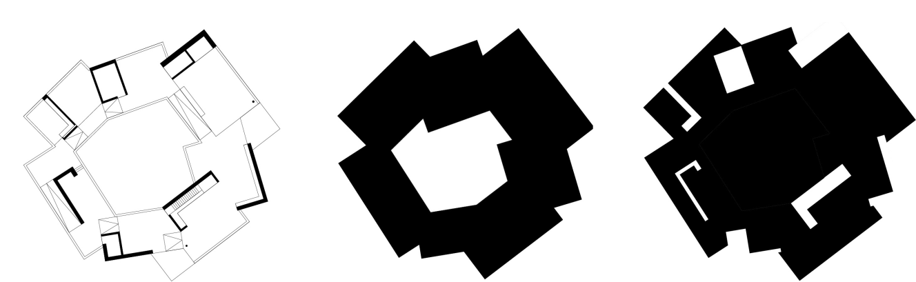
Fig. 8. IN/OUT. Left to Right: Detail Plan, Figureground, and Figured plan, Maggie's Centre, Glasgow, 2011, OMA Case Study Investigation drawings, Present Absence Research Project, 2022-2026, images by Author.
