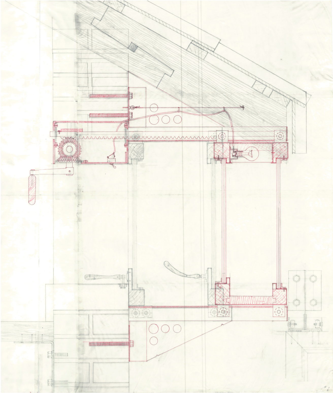
Fig. 4. Seppe Pylyser, Window for a Watchmaker : drawing window detail, scale 1:1. Tracing paper, pencil, thin red marker. Studio Anatomy: [Window] Details , Academic year 2024-2025.
