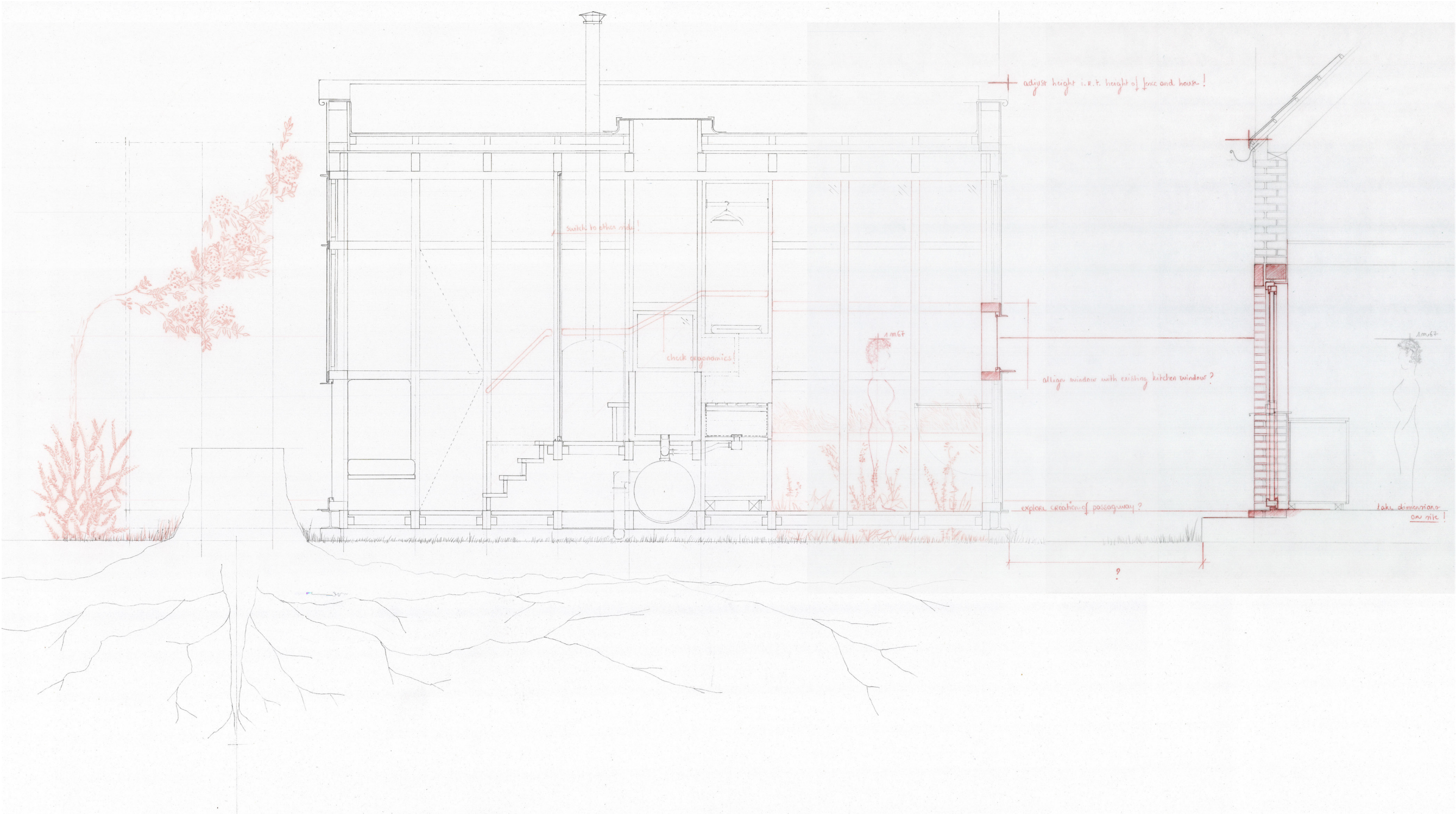
Fig. 10. Longitudinal section indicating some remarks on the initial design of M.'s memorial space (see shared moment 6). Pencil on A2 paper and red pencil on tracing paper. Drawing by Eva Demuynck (2023).
