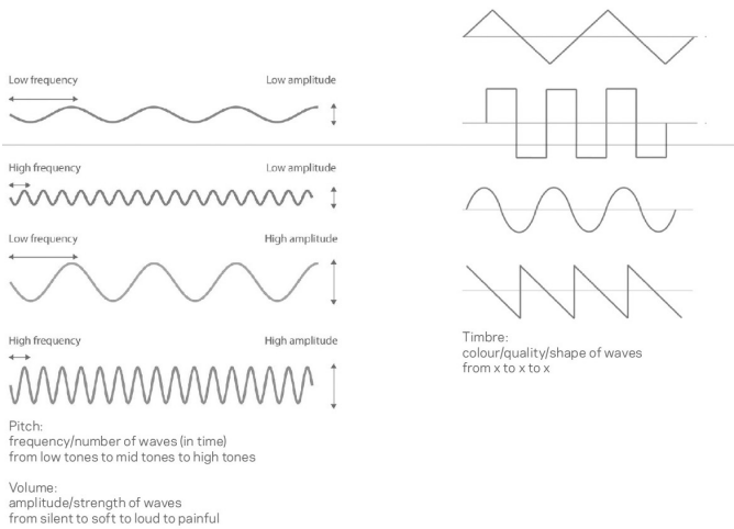
Fig. 4. Pitch corresponds to temporal frequency (Hz), determining perceived tone height; Amplitude reflects sound pressure level, perceived as loudness; Timbre is defined by waveform shape and harmonic content, differentiating sound quality independent of pitch and loudness.
