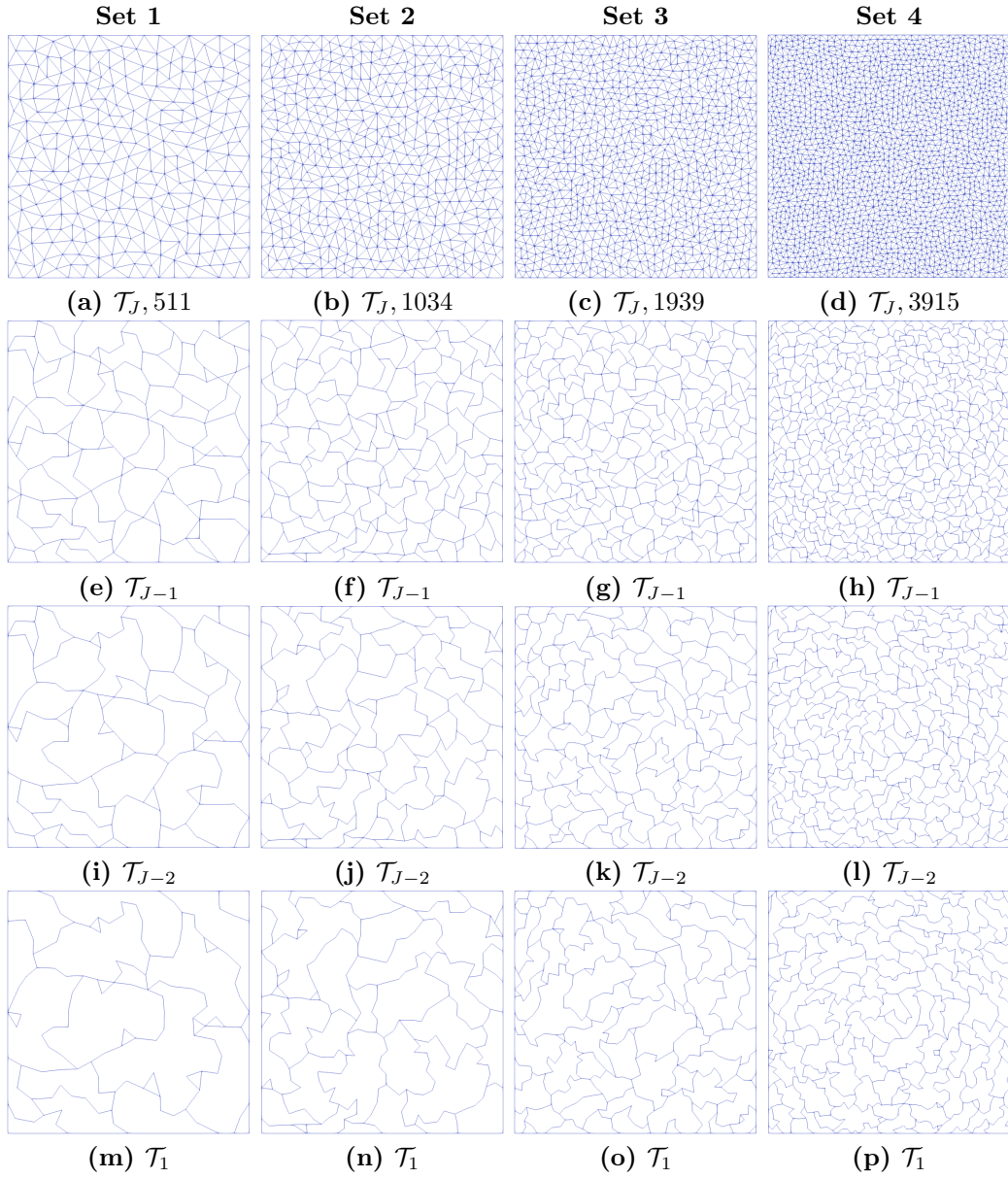
Figure 3: Sequences of agglomerated grids for testing the h-multigrid method. The corresponding fine grids \mathcal{T}_J consist of 511 (a), 1034 (b), 1939 (c) and 3915 (d) elements, respectively.
