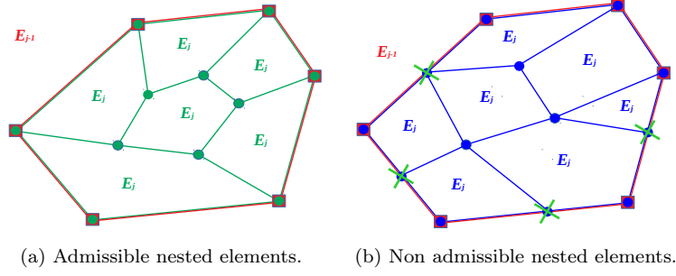
Figure 1: Example of (a) admissible nested elements and (b) non-admissible nested elements. Circles and squares represent the nodes of E_j and E_{j-1} , respectively. The green cross markers in (b) highlight nodes violating the boundary compatibility condition.
