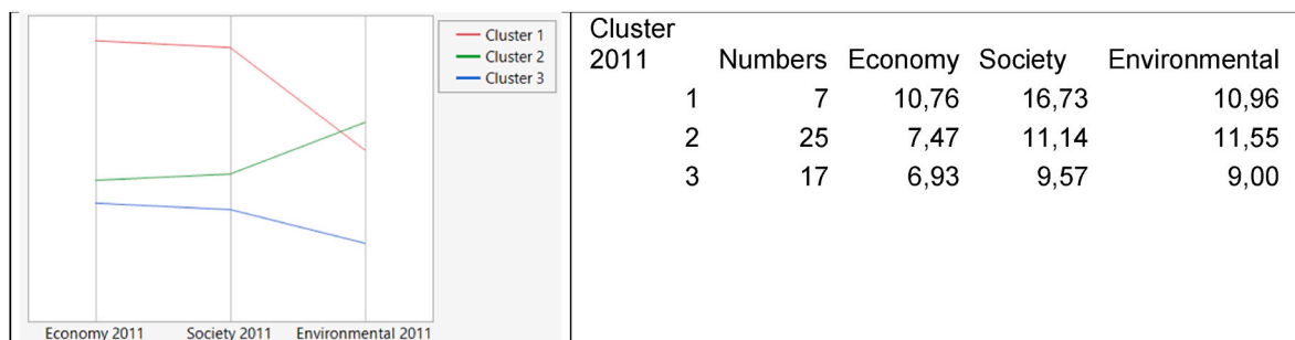
Fig. 1b. Cluster analysis years 2011 Source: Authors' elaboration.
