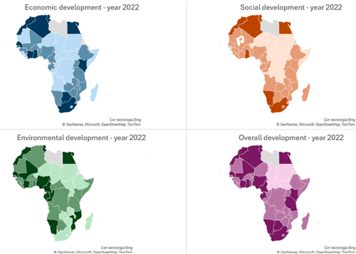
Fig. 2. Geographic patterns in Africa’s dimensions of SDGs and overall performance in 2022.
