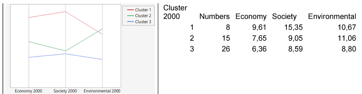
Fig. 1a. Cluster analysis years 2000
