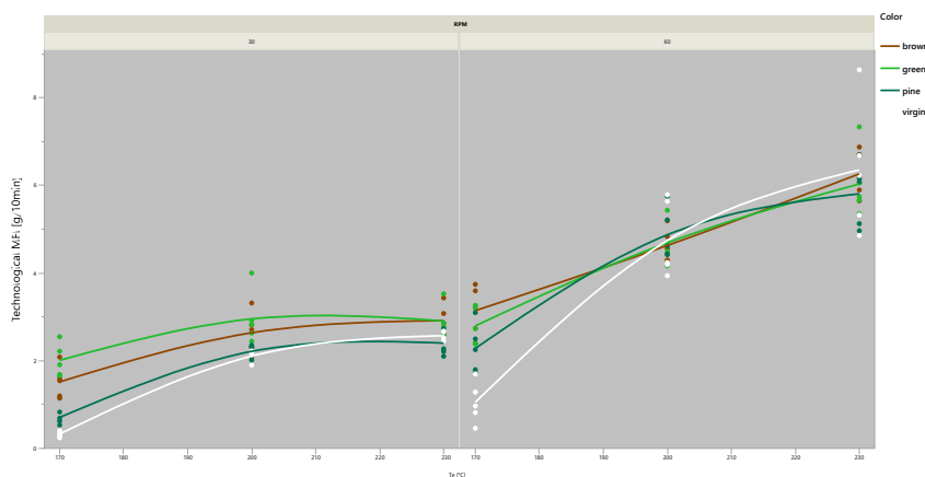
Fig. 2. TMFI response of virgin and recycled polypropylene as a function of T_n (°C) and RPM.
