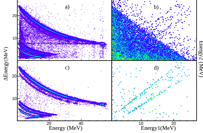
Fig. 1. – (a) \Delta E -E identification scatter plot, raw, energy calibrated data; (b) raw, calibrated energy correlation plot of two signals measured in coincidence into two adjacent strips; (c) same as (a) after the complete pixelation work; (d) same as (b) after the complete pixelation work.
