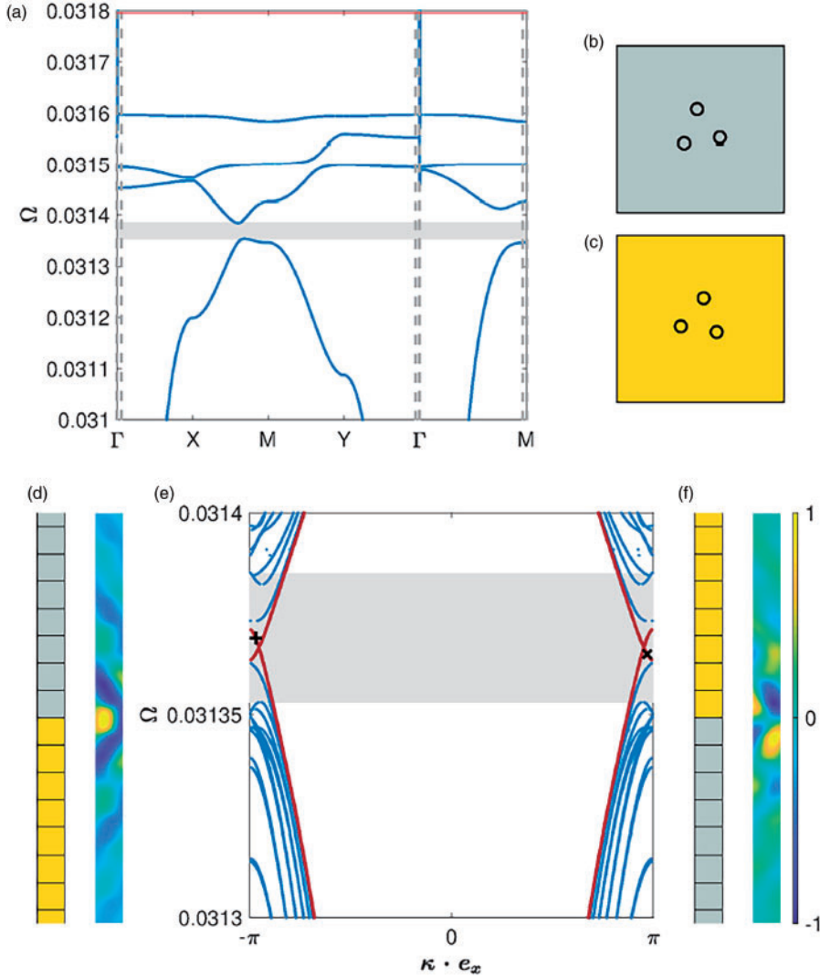
Fig. 8 (a) shows the Floquet-Bloch dispersion branches of the primitive cell in (b). Cells (b) and (c) are obtained by perturbing the arrangement in Fig. 5(c) via rotations of \theta' . By setting \mathbf{X}_{1J} = 0.125 \left[ \cos\left(\frac{2\pi(J-1)}{3} + \frac{\pi}{2} + \theta'\right)\mathbf{e}_x + \sin\left(\frac{2\pi(J-1)}{3} + \frac{\pi}{2} + \theta'\right)\mathbf{e}_y \right] , the grey (b) and yellow (c) cells, respectively correspond to positive and negative rotations in which \theta' = \pm \frac{\pi}{20} . The topological band gap is shaded in grey in (a). (d) and (f) show ribbon media, formed by stacking the chiral pairs in (b) and (c) as shown. The dispersion curves of these ribbon media, obtained from our Floquet–Bloch analysis (D.2), are plotted in (e) where the bulk band gap from (a) is also highlighted in (e). The interfacial modes of interest are plotted in red in (e), the even (d) and odd (f) interfacial states are plotted next to the ribbon media in which they persist; the eigenstates in (d) and (f) correspond to the points \dagger and \times in (e), respectively.
