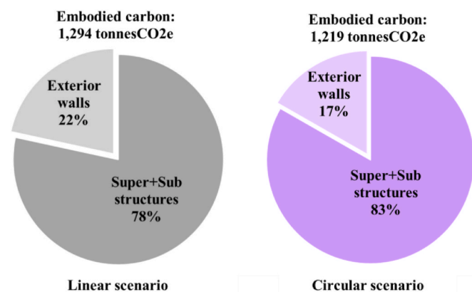
Fig. 9. Embodied carbon emission of the entire building for the linear (left) and circular (right) scenarios, modules A1-A5w, B4, C2–C4.
