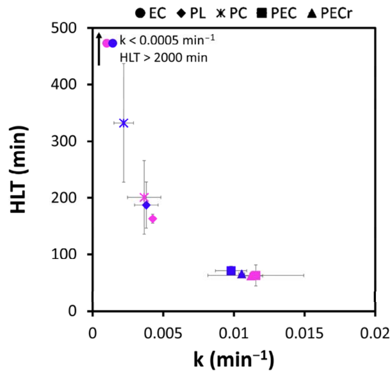
Figure 3. Pseudo first-order kinetic constants k using the Langmuir–Hinshelwood model, and corresponding HLT of EC, PL, PC, PEC, and PECr tests for UV 254 (blue data), and color removal (pink data). Confidence intervals have been calculated based on two replicates.
