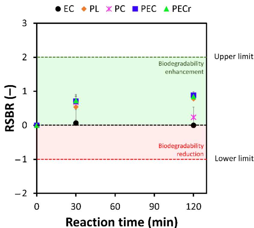
Figure 5. RSBR of EC, PC, PEC, and PECr.
