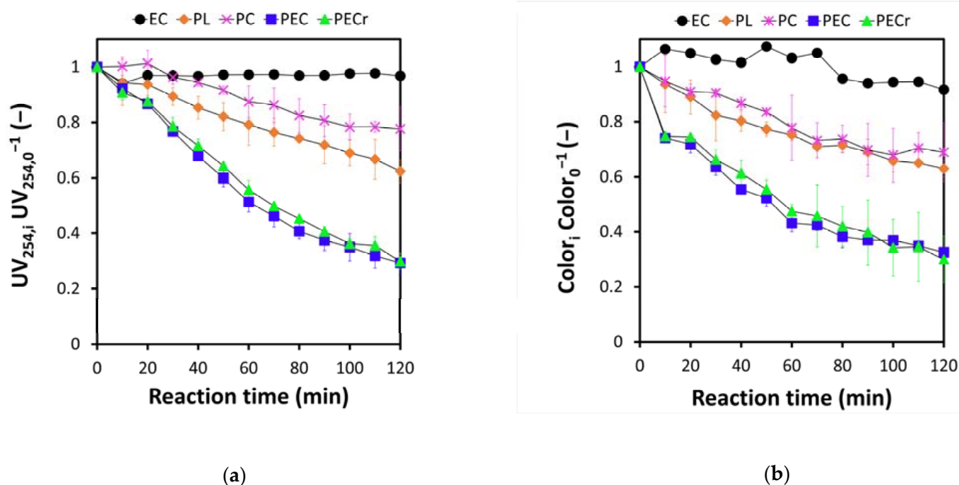
Figure 2. (a) Residual UV_{254} ( UV_{254,i} \cdot UV_{254,0}^{-1} ), and (b) residual color ( Color_i \cdot Color_0^{-1} ) relative to the corresponding parameters at t = 0 during EC, PL, PC, PEC, and PECr tests. Confidence intervals have been calculated based on two replicates.
