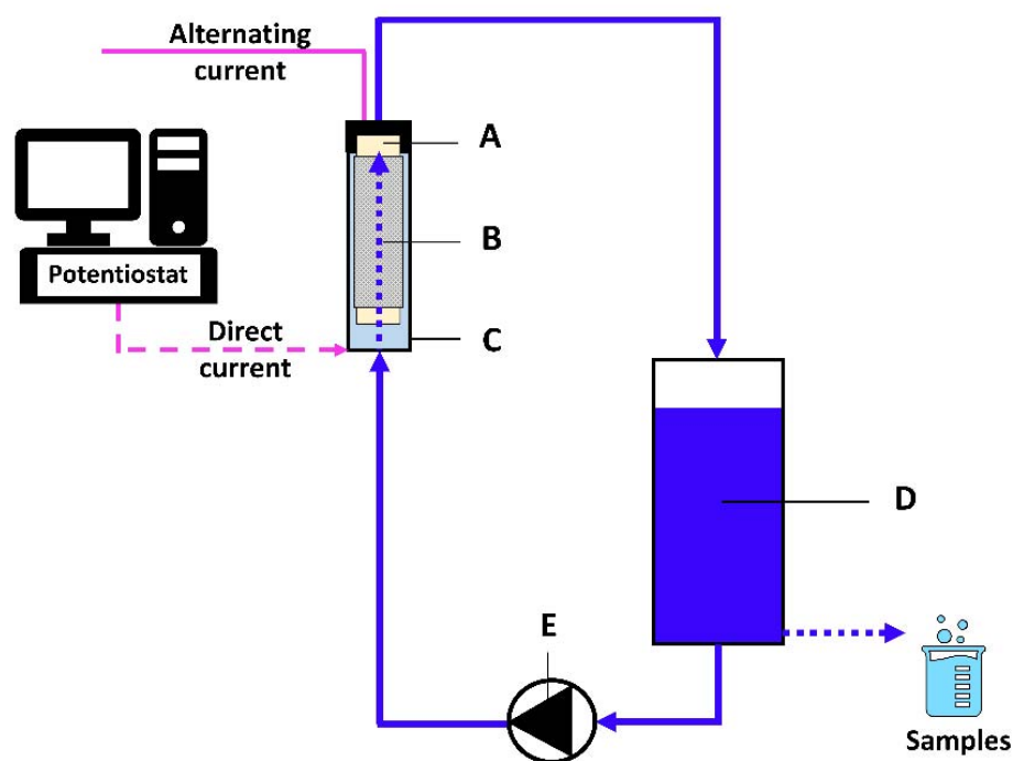
Figure 1. Scheme of the laboratory-scale reactor working in up-flow condition and semi-batch mode. A: lamp, B: \text{TiO}_2 mesh, C: electrochemical reactor, D: tank, and E: pump.
