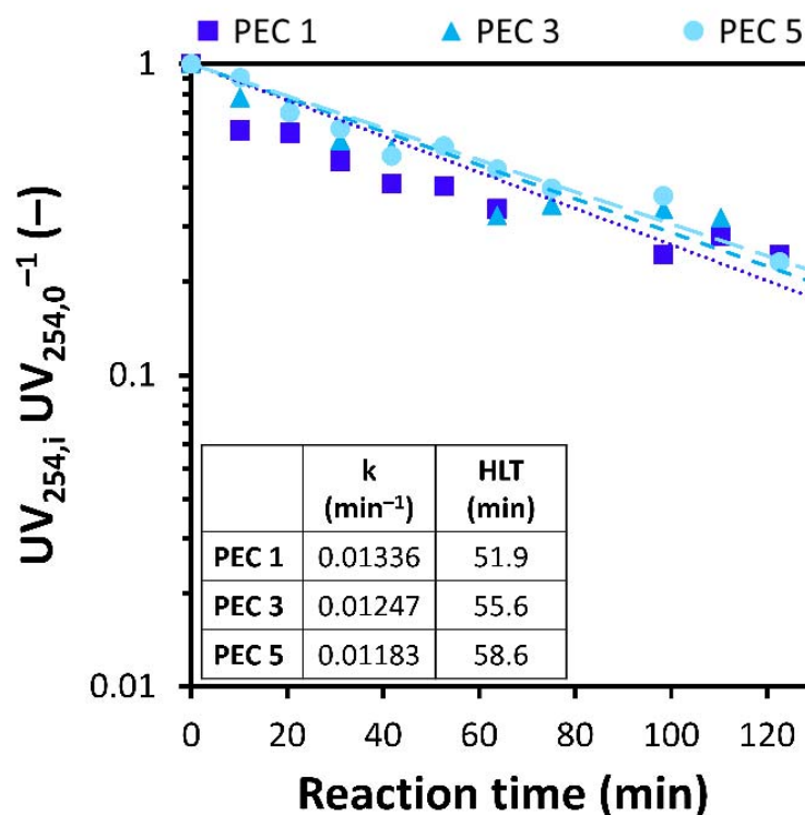
Figure 6. Aging effect of the nanostructured TiO 2 meshes under repeated use in PEC process. PEC 1, PEC 3, and PEC 5 represent the UV 254 removal after one, three, and five-time use.
