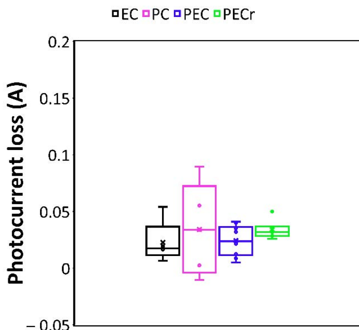
Figure 7. Photocurrent loss of the \text{TiO}_2 mesh after one test (reaction time: 2 h). Confidence intervals have been calculated based on five replicates.
