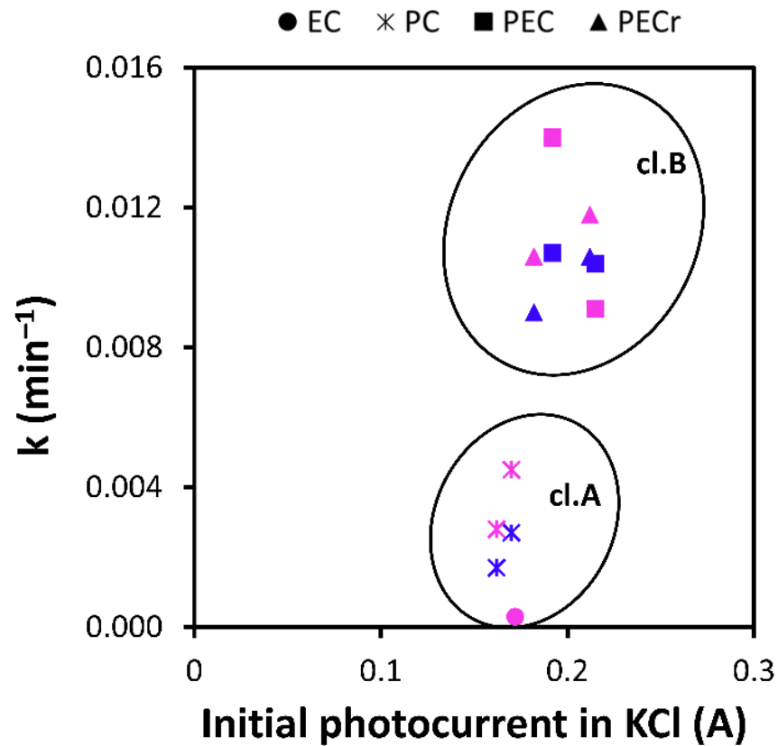
Figure 4. Initial photocurrent and first-order kinetic constants using the Langmuir–Hinshelwood model of EC, PC, PEC, and PECr for UV 254 (blue data), and color removal (pink data). cl: cluster.
