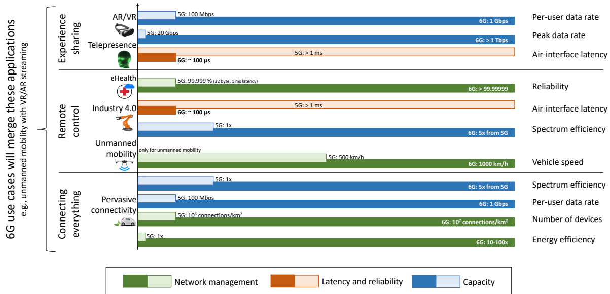
Fig. 2: Representation of multiple KPIs of 6G use cases, together with the improvements with respect to 5G networks, using data from [1]–[9].
