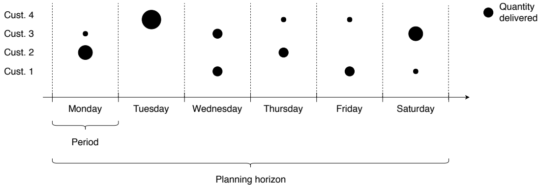
Figure 2: Inventory Routing Problems: an example.
