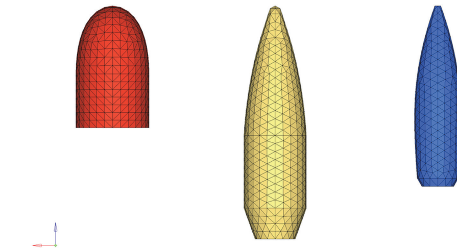
Figure 8: Finite element models of the bullets, left to right: 9x21mm FMJ round nose (red), 7.62x39mm FMJ (yellow), 5.6x45mm NATO (blue).
