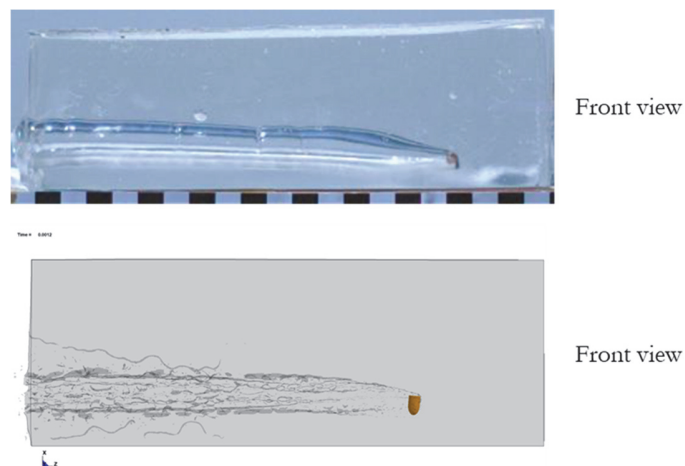
Figure 12: 9x21mm FMJ round nose impact. Comparison between experimental results (above) and simulation (below). Time = 1.2 ms. The resolution of the checkered ruler is 20 mm.
