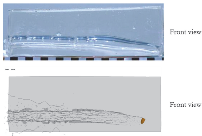
Figure 13: 9x21mm FMJ round nose impact. Comparison between experimental results (above) and simulation (below). Time = 1.6 ms. The resolution of the checkered ruler is 20 mm.
