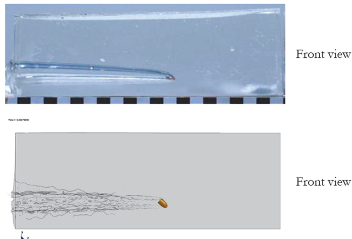
Figure 11: 9x21mm FMJ round nose impact. Comparison between experimental results (above) and simulation (below). Time = 0.8 ms. The resolution of the checkered ruler is 20 mm.
