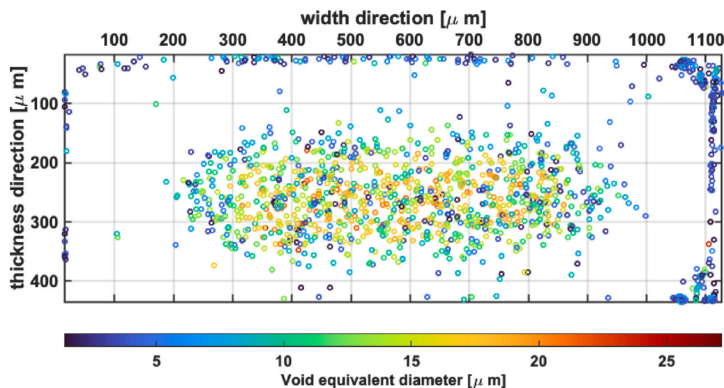
Fig. 7. Spatial distribution of pores, color map refers to pore diameter [ \mu\text{m} ].
