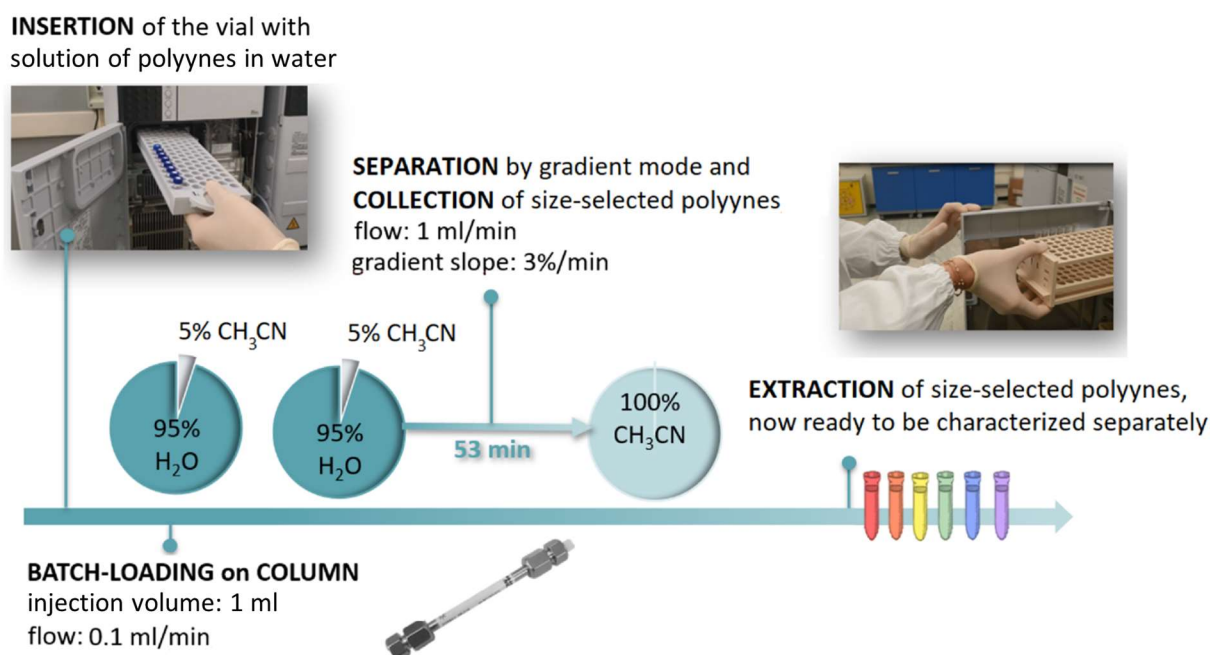
Figure 2 – Key steps of our single RP-HPLC procedure: insertion of aqueous polyynes solution in RP-HPLC system, batch-loading on-column concentration method, separation by gradient method, and collection of size-separated polyynes and extraction of the fractions.
