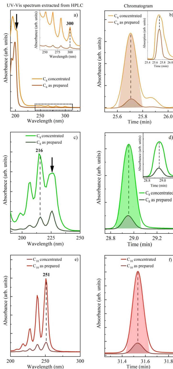
Figure 4 - UV-Vis spectrum (on the left column) extracted from DAD of RP-HPLC and the corresponding chromatographic peak (on the right column) at the wavelength indicated in the UV-Vis spectrum for the case of C_6 , C_8 , and C_{10} before and after our single RP-HPLC procedure. The area considered to calculate the increments of C_6 , C_8 and C_{10} are colored. Insets: low-intensity absorption peaks of C_6 (panel a), the chromatographic peak of C_6 selected at 199 nm (panel b) and the chromatographic peak of C_8 selected at 225 nm (panel d).
