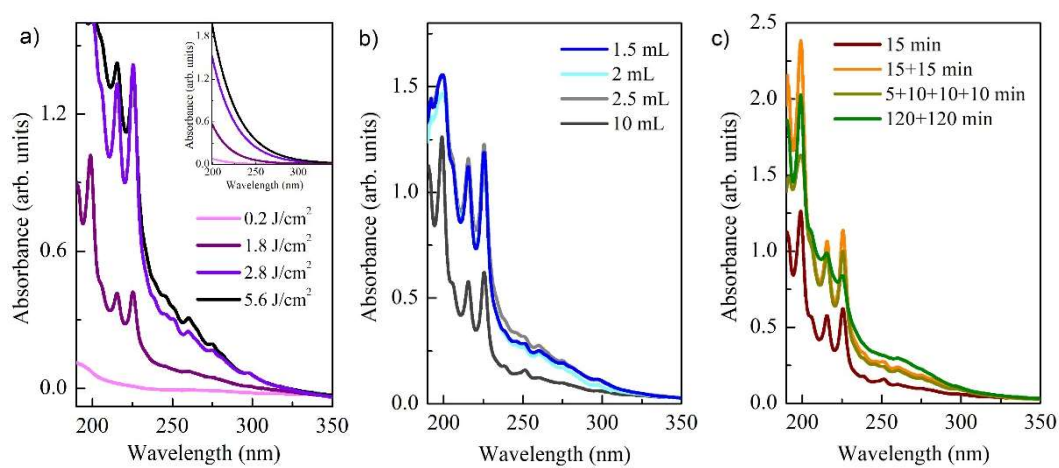
Figure 1 – UV-Vis absorption spectra (range: 190-350 nm) of polyynes mixture with main UV-Vis peak of hydrogen-capped polyynes (C 6 , C 8 , C 10 ) marked a ) at different fluences (0.2, 1.8, 2.8, 5.6 J/cm 2 ), fixed water volume (2 ml) and ablation time (15 min), b ) at different liquid volumes (1.5, 2, 2.5, 10 ml), fixed fluence (2.8 J/cm 2 ) and ablation time (15 min) and c ) at different ablation times (15 min, 30 min with a break of 2 min after 15 min, 35 min with breaks of 2 min after 5, 15 and 25 min, 240 min with a break of 2 min after 120 min), fixed fluence (2.8 J/cm 2 ) and water volume (2ml). In the inset, the fitting exponential curves of the background of each spectrum at different fluences (0.2, 1.8, 2.8, 5.6 J/cm 2 ).
