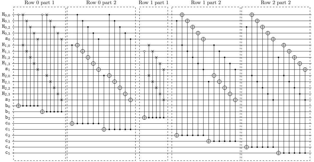
Fig. 4. Basic quantum circuit employed to perform the Gauss-Jordan Elimination on the augmented matrix [\tilde{H} \mid \mathbf{s}] having r = 3 and n = 4 . The quantum register containing the elements of the parity-check permuted matrix is denoted by H , while the one containing the elements of the syndrome is denoted by s . b and c are the registers associated to the two vectors \mathbf{B} and \mathbf{C} employed in Algorithm 3.
