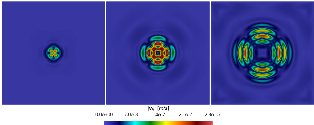
Figure 6: Test case 1: computed velocity field |\mathbf{v}_h| at the time instants t = 0.2 s (left), t = 0.4 s (center), t = 0.6 s (right).
