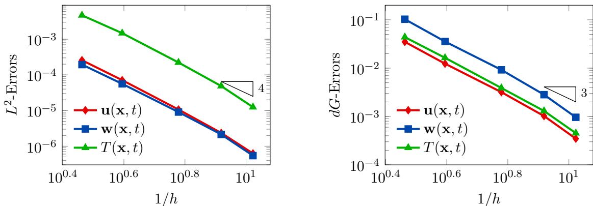
Figure 2: Convergence test for \tau = 0 : computed errors in L^2 -norm (left) and dG -norm (right) versus 1/h ( \log - \log scale). The errors are computed at the final time T_f . The polynomial degree of approximation is taken as \ell = 3 .
