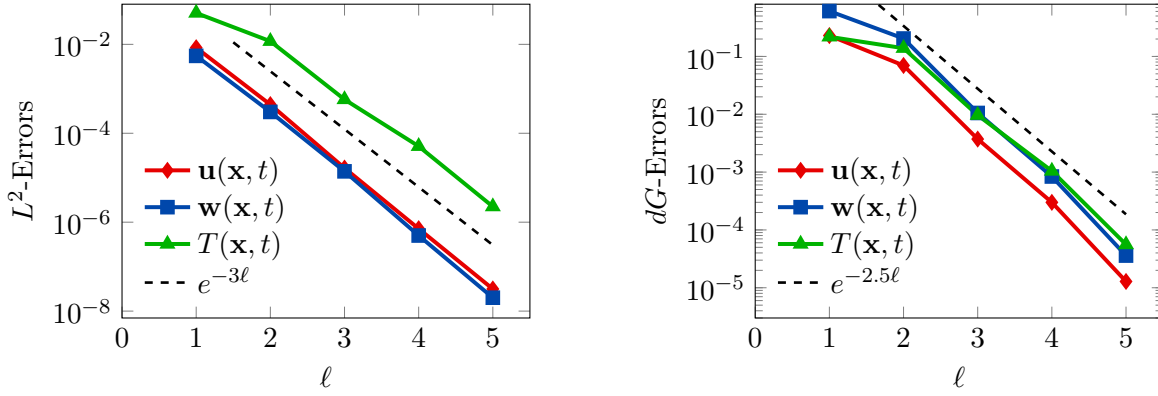
Figure 4: Convergence test for \tau = 0.01 : computed errors in L^2 -norm (left) and dG -norm (right) versus \ell ( semi-log scale). The errors are computed at the final time T_f . The computational mesh is made of 100 polygons.
