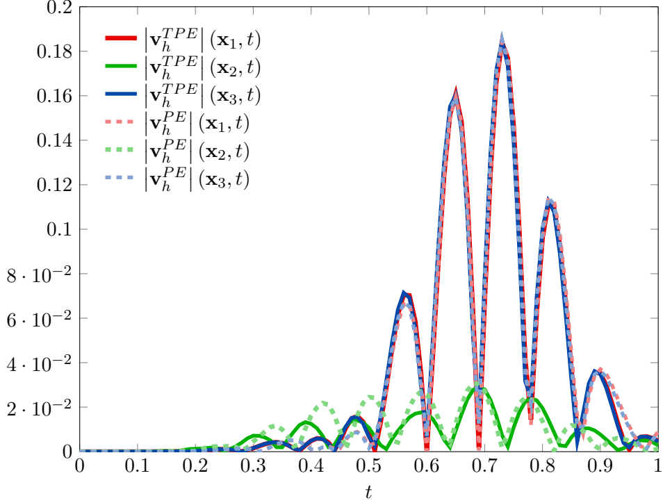
Figure 12: Test case 2: comparison of time-evolution of the solid velocity |\mathbf{v}_h| measured in the points \mathbf{x}_2 (green), \mathbf{x}_3 (blue), and \mathbf{x}_1 (red) for the thermo-poroelastic (TPE) model (solid-line) and the poroelastic (PE) one (dashed-line). Unit of measure: \mu\text{m s}^{-1} .
