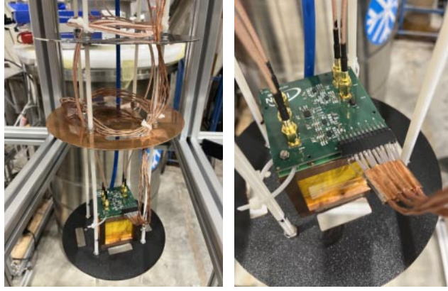
Fig. 4. – Close-up pictures of the NaI(Tl) crystal coupled with SiPM array and front-end electronics.
