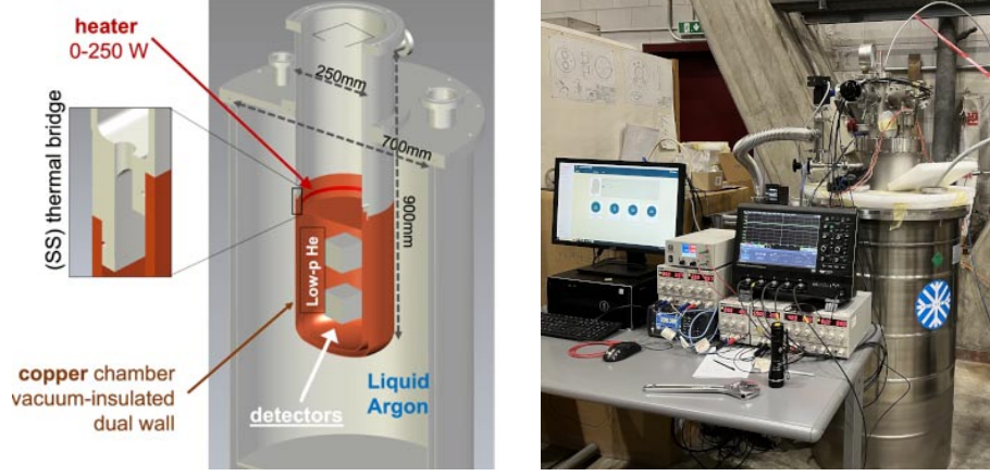
Fig. 1. – Cryostat CAD model (left); picture of the cryostat set-up at the LASA in Milan (right).
