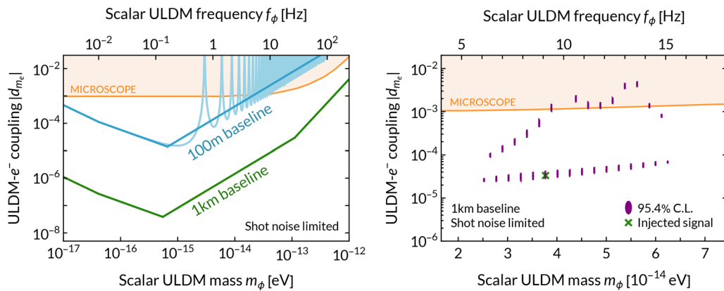
Fig. 5. Left panel: projections for sensitivities to scalar ULDM linearly coupled to electrons (shot noise limited and assuming \text{SNR} = 1 ). The lighter-blue 100 m baseline curve shows the oscillatory nature of the sensitivity projections, while the darker-blue and green curves show the envelope of the oscillations. Right panel: parameter reconstruction, adapted from with permission from Badurina et al. , “Super-Nyquist ultralight dark matter searches with broadband atom gradiometers,” arXiv:2306.16477. Copyright 2023 Authors, licensed under a Creative Commons Attribution Unported License, 77 of an injected signal with f_\phi = 9.1 Hz and d_{m_e} = 3.7 \times 10^{-5} (green cross) for a 1 km baseline assuming a constant sampling frequency of 0.3 Hz. The purple contours show the islands of parameter space compatible with the signal at 95.4% C.L. In both panels, the shaded orange region shows constraints from MICROSCOPE as described in Refs. 78 and 79.
