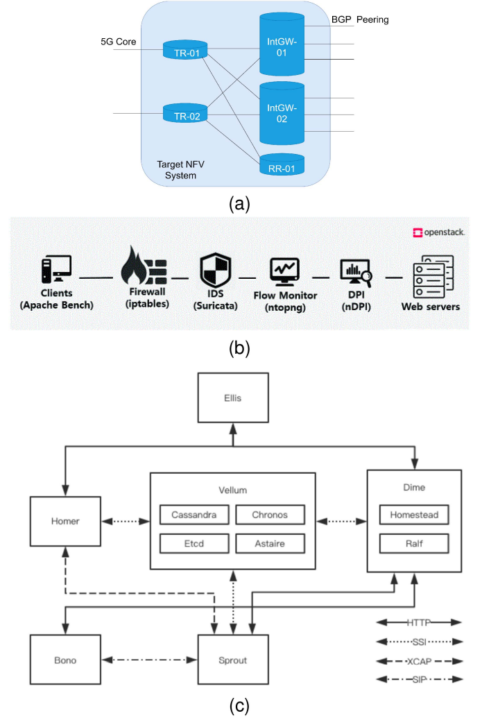
Fig. 2. NFV system of (a) ITU Dataset, (b) MEC Dataset [27], and (c) IMS Dataset [6].
