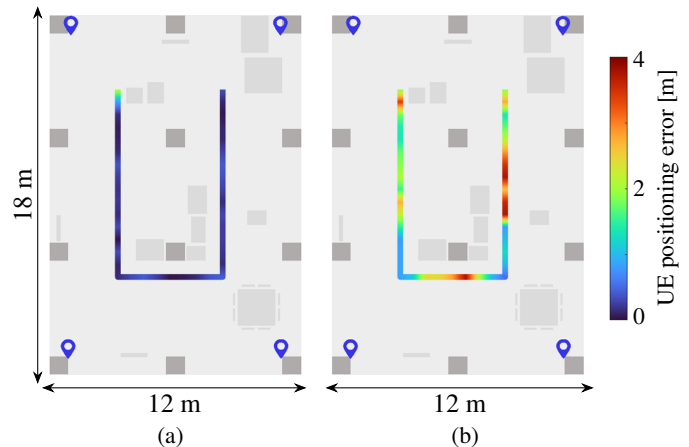
Fig. 32. Indoor mobile positioning - heatmap of the positioning error using DL-TDOA measurements. (a) EKF with NLOS detection; (b) EKF without NLOS detection.
