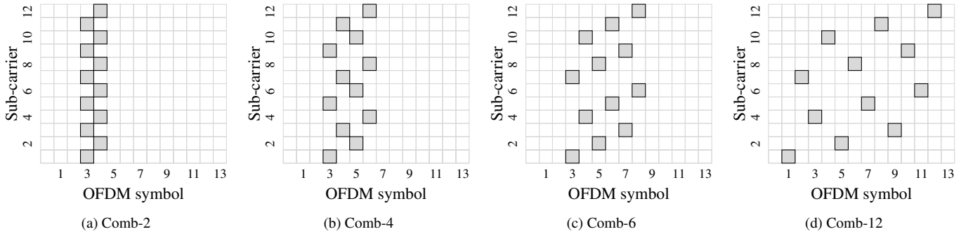
Fig. 11. Representation of four different PRS time/frequency comb patterns, as described by 3GPP Rel-16 [89], [361].
