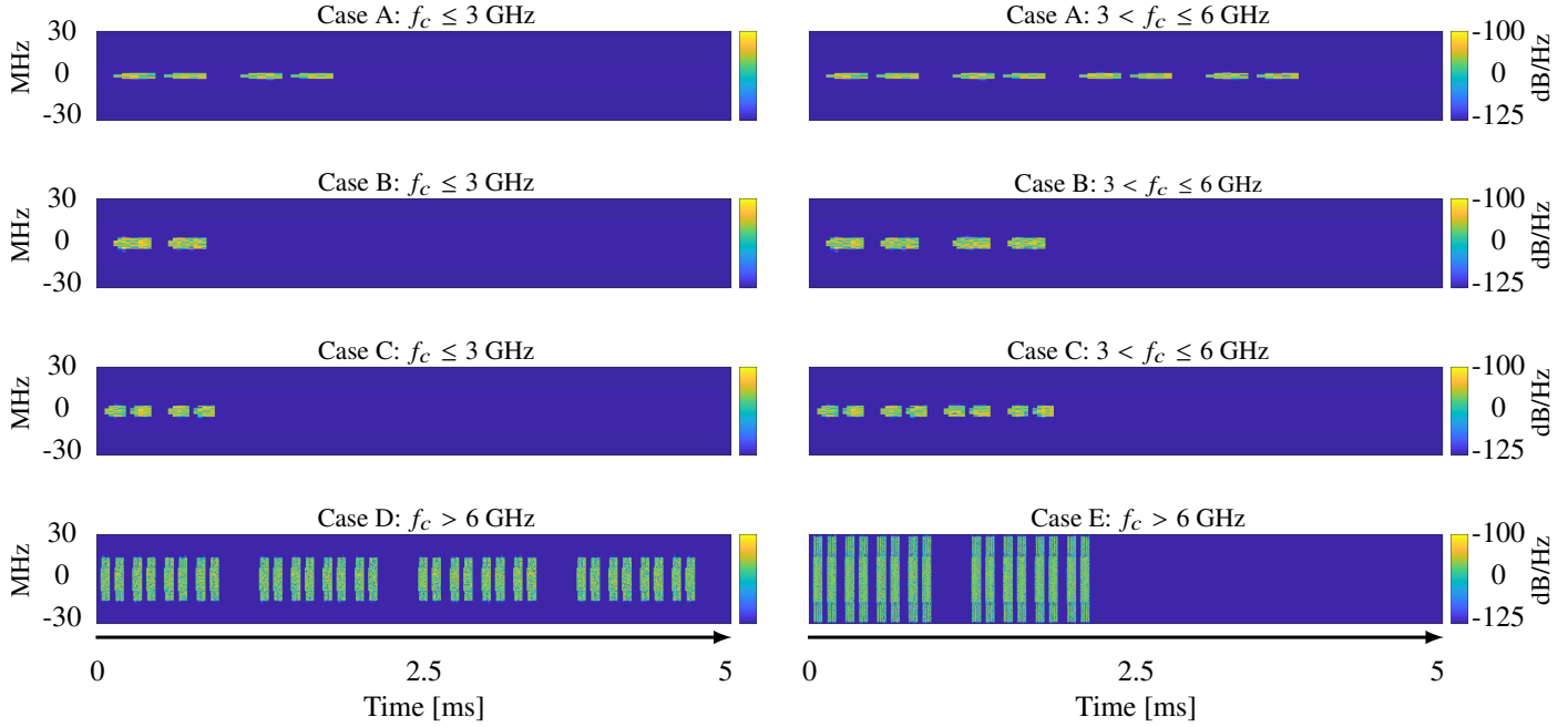
Fig. 10. SSB pattern cases according to the different carrier frequency, as described by 3GPP Rel-15 [358], [359].
