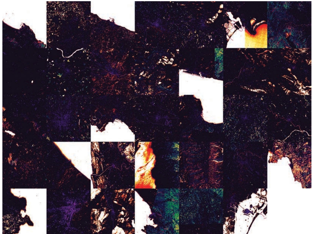
Fig. 9. False colour galaxy-like images mosaic of the thirty-three locations; the images are sorted in location name alphabetical order from left to right and up to the bottom.
