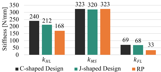
Fig. 16. Assessment of the design solutions of the C-shaped and J-shaped prostheses with respect to the RP in terms of the stiffnesses at the critical stance-phase stages ( k_{HL} , k_{MS} , and k_{FL} ).
