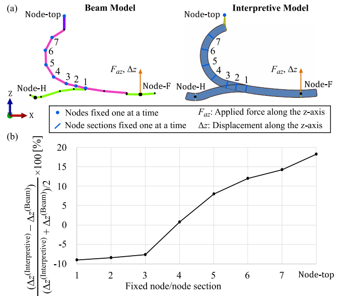
Fig. 18. The effect of the C-shape on the difference between the beam and the plane stress FE models in terms of stiffness prediction. a) Description of the loading conditions applied for making the comparison, and b) the percent difference of the estimated \Delta z at node-F given one fixed node/node section at a time.
