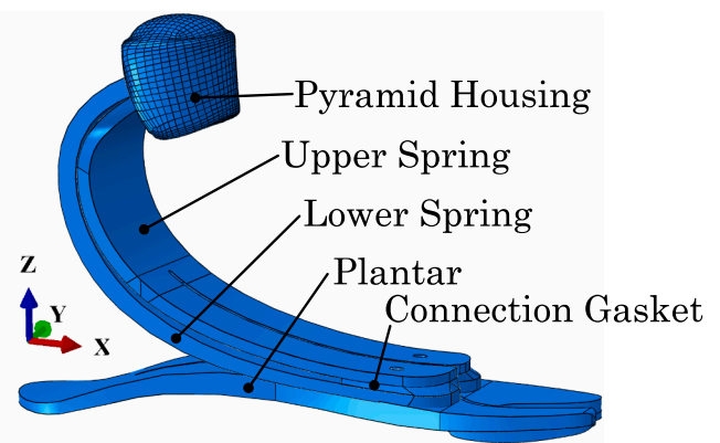
Fig. 1. The RP solid model with the main parts pointed out.
