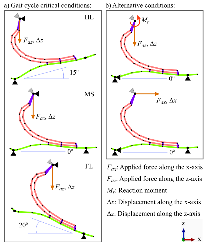
Fig. 3. BC, loads, and orientations imposed in beam FE model for the computation of prostheses stiffness at a) the maximum heel loading condition ( k_{HL} ), Mid-stance ( k_{MS} ), and maximum forefoot loading condition ( k_{FL} ), in addition to b) the vertical and horizontal stiffnesses ( k_z and k_x ), and reaction moment factor ( Q_m ).
