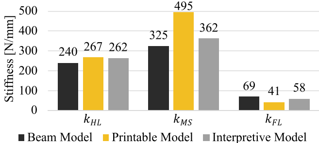
Fig. 17. Assessment of the designed prosthesis beam FE model with respect to the plane stress FE models shown in Fig. 8 in terms of the stiffnesses at the critical stance-phase stages ( k_{HL} , k_{MS} , and k_{FL} ).
