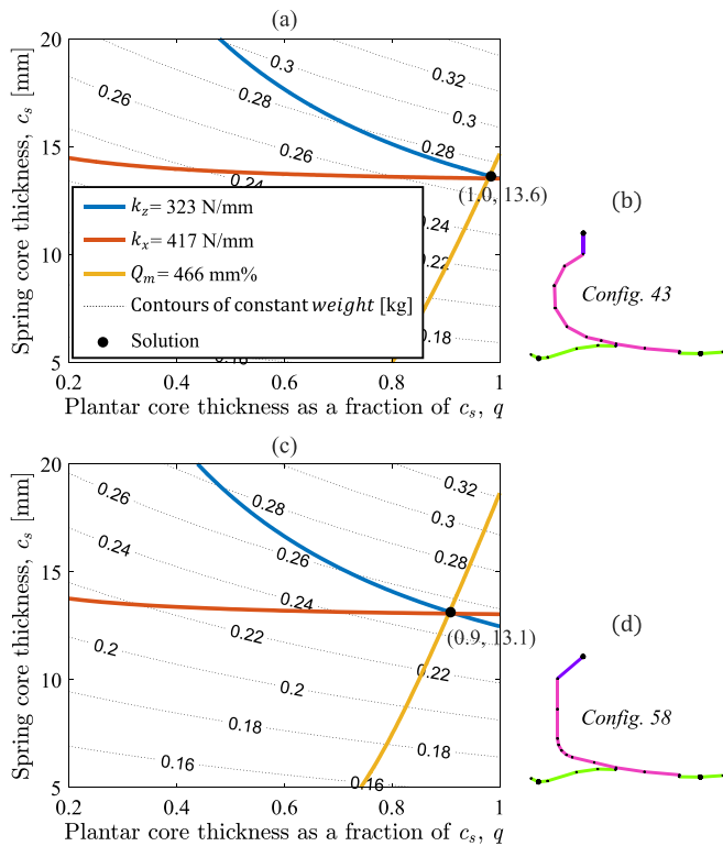
Fig. 15. Solutions of design case II, defined in Fig. 9b, where the design chart (a) corresponds to b) Config. 43 of the C-shaped prosthesis, and the design chart (c) corresponds to d) Config. 58 of the J-shaped prosthesis at which the solutions were found.
