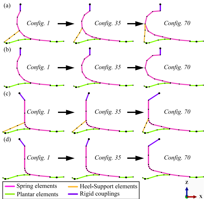
Fig. 6. Illustration of the variation between the spring configurations for the a) C-shaped prosthesis with a heel-support and b) without, and the c) J-shaped prosthesis with a heel-support and d) without.
