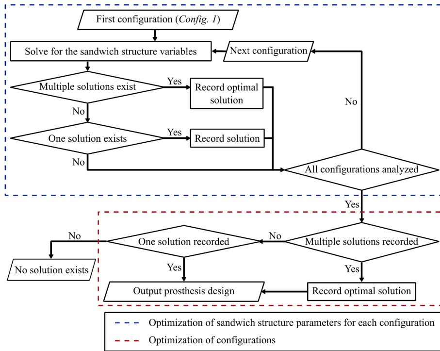
Fig. 10. Flowchart of the design framework applied in the optimization tool developed through MATLAB. The first and the second phases of optimization are distinguished by the blue and red dashed rectangles, respectively.
