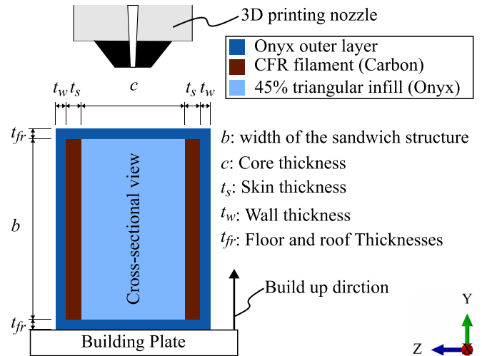
Fig. 7. Schematic of the 3D printing strategy relative to the novel prosthesis material structure.
