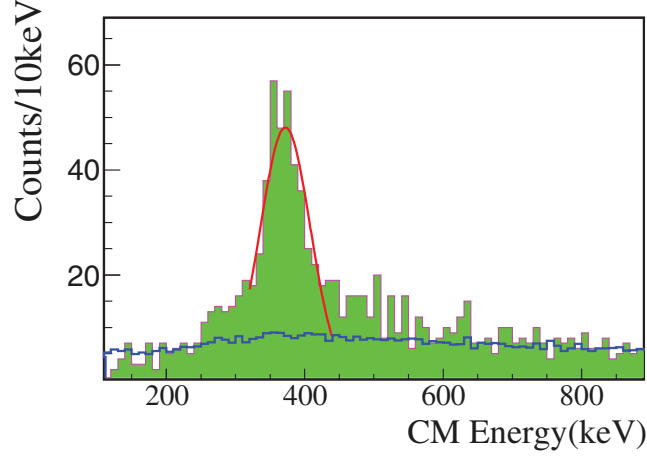
Fig. 2. – The Hoyle state resonance measured in 3- \alpha -particles coincidences. The red line is a Gaussian fit of the resonance. The blue line is the background computed with the event mixing technique.
