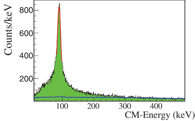
Fig. 1. – The {}^8\text{Be}_{g.s.} resonance measured in 2- \alpha -particles coincidences. The red line is a Gaussian fit of the resonance. The blue line is the background computed with the event mixing technique.
