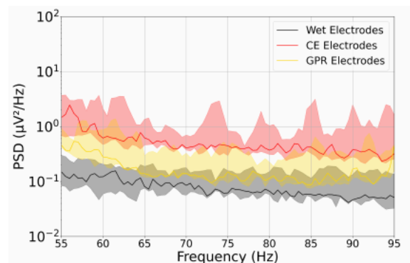
Figure 3: Comparison of Power Spectral Density (PSD) for frequencies above 55Hz between CE, GPR, and wet electrodes. PSD is reported on a logarithmic scale, with median IQR shown for each electrode type.
