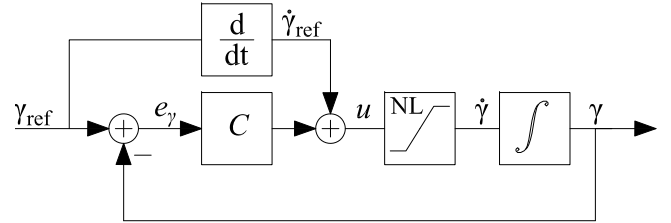
Fig. 2: Proposed delay-recovering loop scheme.
