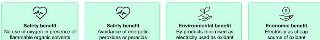
Scheme 29 Batch vs. continuous-flow approach for thioether oxidation. The traditional methods (a) rely on oxygen/peroxides, or metal-based oxidants to obtain the sulfone, leading to safety risks, hazardous byproducts, and higher costs. The continuous-flow electrochemical approach (b) replaces these reagents with electricity as the oxidant, eliminating energetic peroxides, minimizing waste, and avoiding flammable oxygen-solvent mixtures. Adapted from ref. 450.
