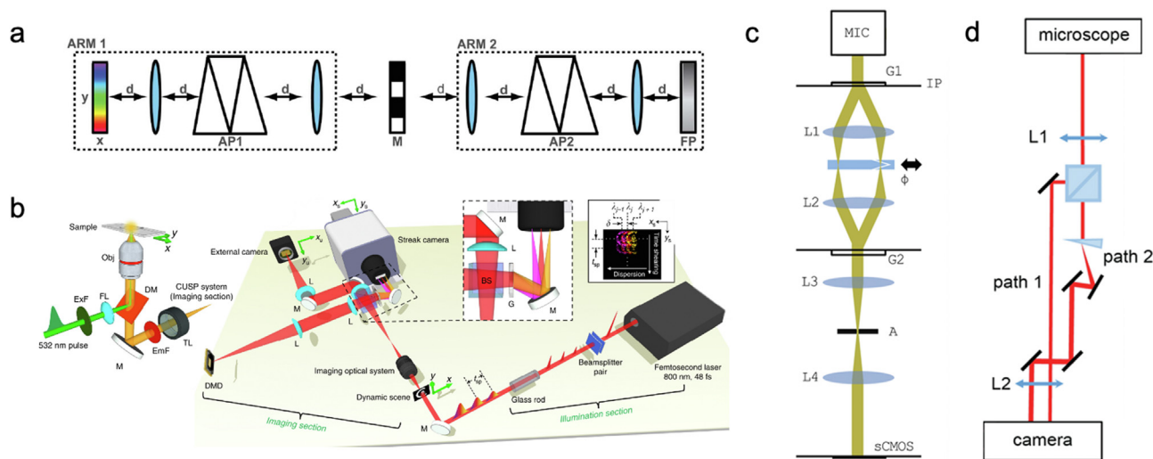
Fig. 5. Four different methods to perform a spectrally resolved compressive fluorescence microscopy: (a) CASSI, reprinted with permission from (Cull et al., 2010) © The Optical Society; (b) CUSP. Left: illumination section for the microscope. Right: complete CUSP setup. Adapted from (Wang et al., 2020) under a Creative Commons Attribution 4.0 International License ( http://creativecommons.org/licenses/by/4.0/ ); (c) IFTS, adapted with permission from (Wadduwage et al., 2017) © The Optical Society; here two diffraction gratings (G1 and G2) generate the interferometer and a variation of the thickness of a glass block is used to introduce a path length difference. An aperture (A) is introduced to block off-axis orders. (d) Space-constrained computational spectral imaging detection system. Adapted with permission from (Wang et al., 2019) © The Optical Society.
