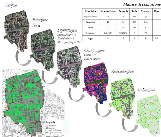
Fig. 17 - Abstract grafico della routine creata per la classificazione delle aree impermeabilizzate in area urbana / Graphical abstract of the automated routine created to classify paved surfaces in the study area (Source: Authors' elaboration).
