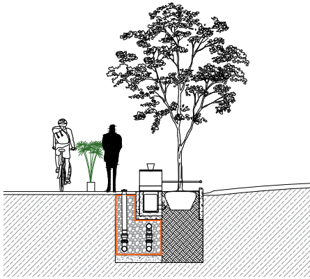
Fig. 50 - Planter ibrido con attrezzatura tipo B1 / Hybrid planter with type B1 equipment (Source: Authors' elaboration).
