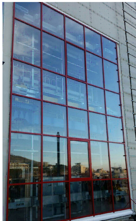
Fig. 24 - Campione sottoposto a prova nell'assetto sperimentale: Full Scale Mock-Up / Sample tested in the experimental setup: Full Scale Mock-Up (Source: Authors' elaboration).
