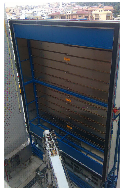
Fig. 28 - Vista della Camera termica / Thermal chamber view (Source: Authors' elaboration).
