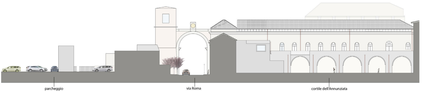
Fig. 17b - Profilo di rilievo ambientale / Environmental survey section (Source: Authors' elaboration).
