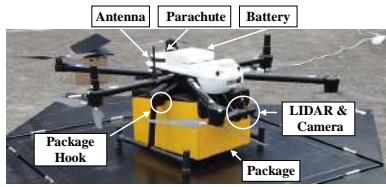
Figure 9: The delivery drone used for evaluation. Besides the speakers, the rest of the drone equipment is part of a standard drone configuration and would be present anyways on any professional-grade drone platform.
