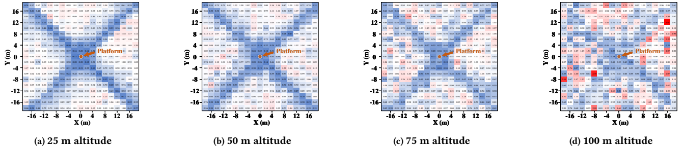
Figure 12: Heatmaps of localization error on the horizontal plane at different altitudes.
