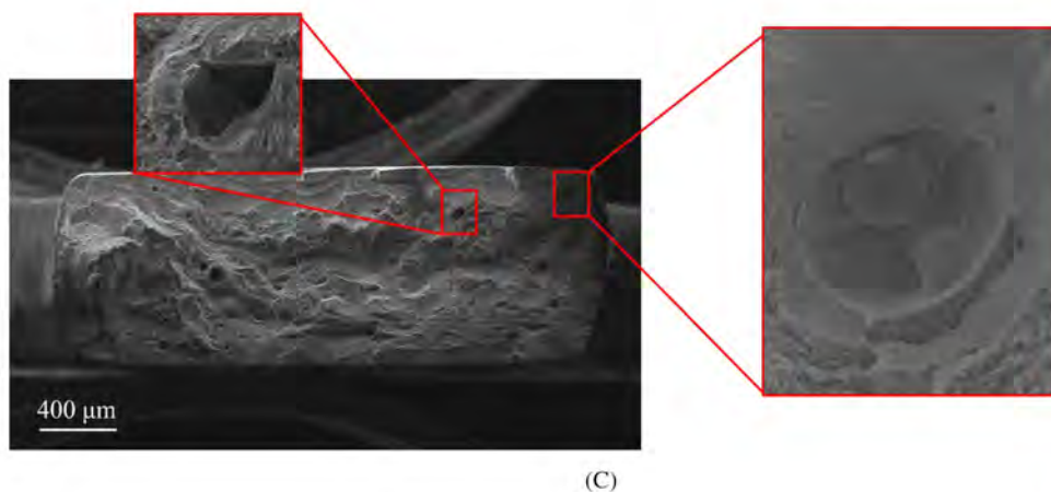
FIGURE 3 AlSi10Mg tensile curve obtained from dogbone specimens printed at different printing angles and with different surface qualities (A, polished surface; B, as-built surface); (C) SEM images of fracture surface of Sample 2, highlighting the presence of internal defects on the fracture surface [Colour figure can be viewed at wileyonlinelibrary.com ]
