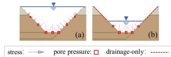
Figure 4. Schematization of the boundary conditions: (a) at the end of excavation; (b) at the end of the dewatering.
