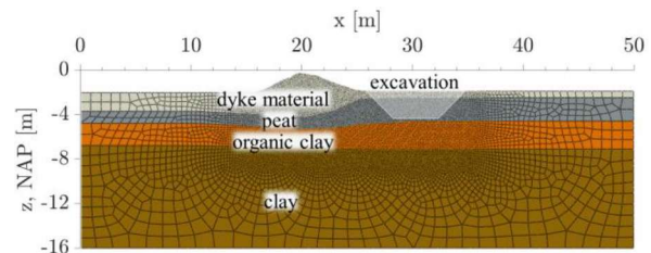
Figure 3. Geometry and mesh of the FE model.
