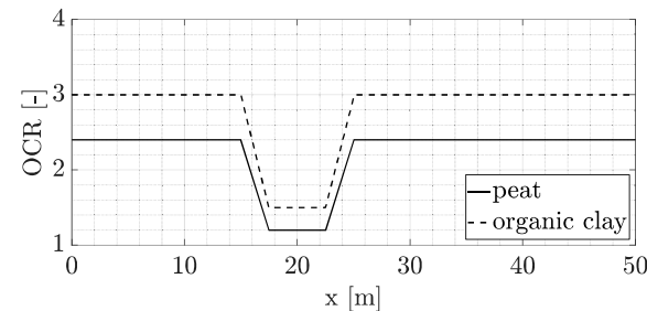
Figure 5. OCR profile in peat and organic clay layer.
