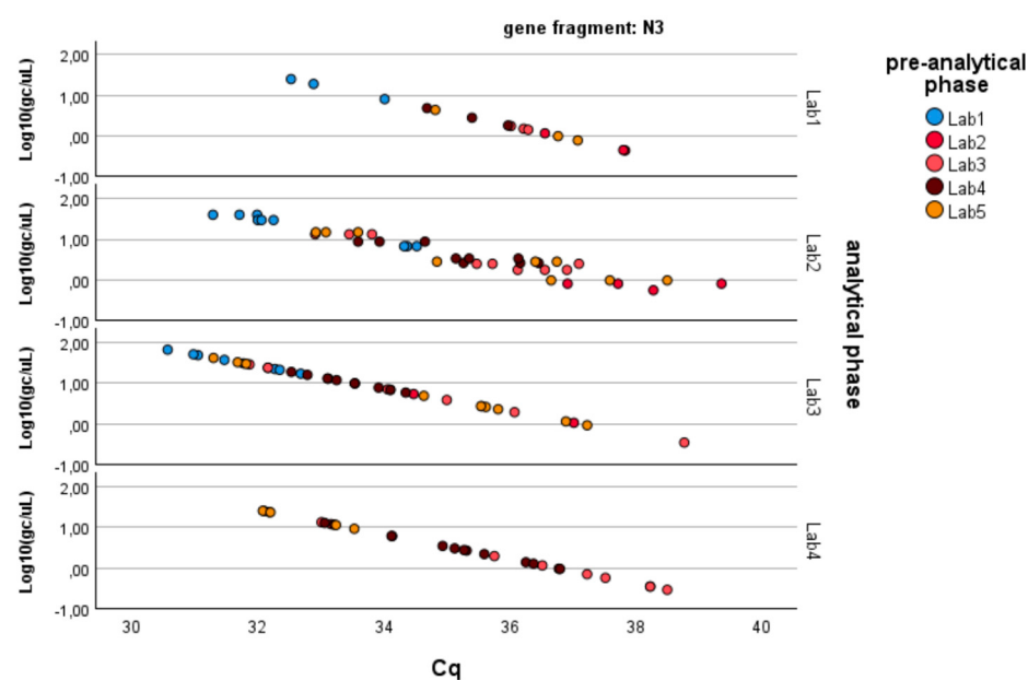
Figure 4. Log-transformed detections of N3 gene fragment copies/ \mu\text{L} concentration: differences among laboratories concerning the analytical and pre-analytical phases. Full regression statistics for the linear relationship depicted in the chart are provided in Table S3.
