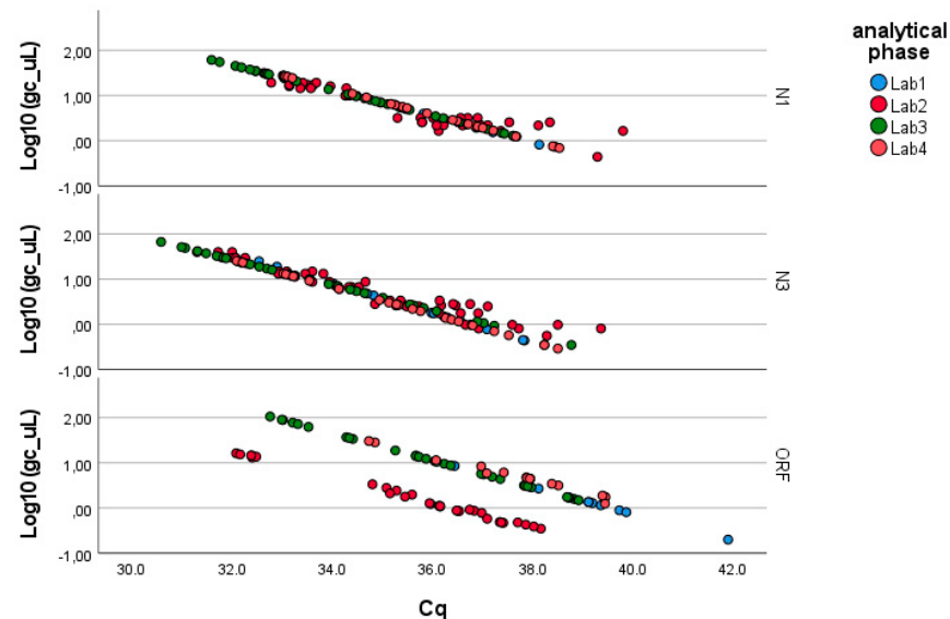
Figure 2. Linearized relationships of the log-transformed concentrations (g.c./μL) across the laboratories responsible for the analytical phase. Full regression statistics for the linear relationship depicted in the chart are provided in Table S1.
