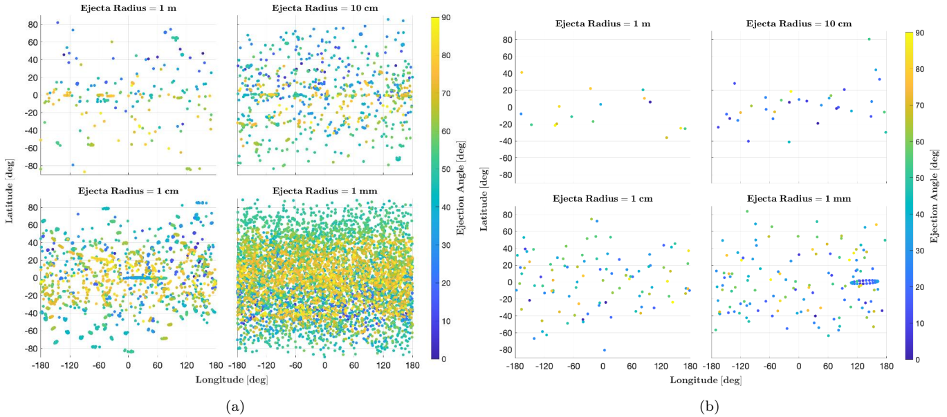
Figure 13. The distribution of ejection location for ejecta following the stable manifold of the terminator orbits and impacting the surface of (a) Didymos and (b) Dimorphos.
