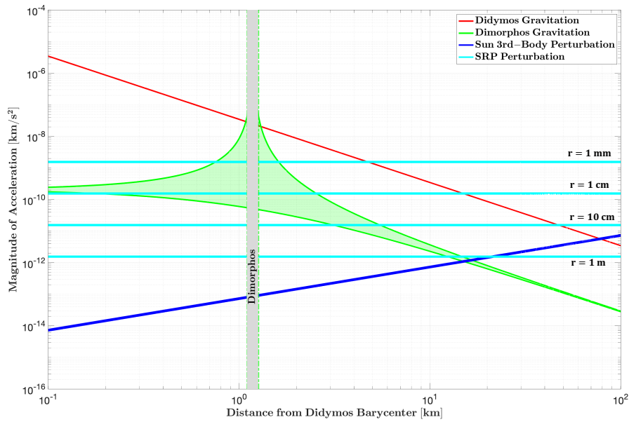
Figure 1. Acceleration environment in the vicinity of the Didymos binary system. The x -axis indicates the radial distance along the line extending from the Didymos barycenter toward the Dimorphos barycenter. The ranges between minimum and maximum accelerations caused by the gravitation of homogeneous spherical Didymos and Dimorphos, third-body gravitational perturbation from the Sun, and SRP on spherical ejecta of varying radii are presented. These ranges are calculated over a time frame spanning from the DART impact on 2022 September 26 to 60 days postimpact. During the investigated period, the Sun–Didymos distance remains relatively stable, with a maximum variation of 3.16%. Therefore, the minimum and maximum perturbing accelerations from the Sun are on the same order of magnitude, leading to an almost invisible blue shaded area in the figure.
