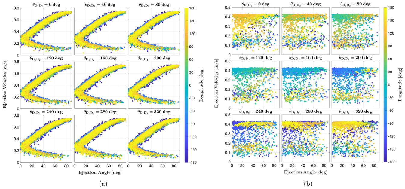
Figure 8. The distribution of ejection velocity, angle, and location for ejecta following the stable manifold of the planar Lyapunov orbits and impacting the surface of (a) Didymos and (b) Dimorphos.
