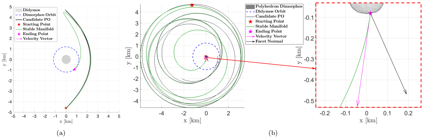
Figure 11. An example of a backward-propagated ejecta trajectory along the stable manifold of a planar Lyapunov orbit eventually impacting Dimorphos. (a) Trajectory in the Didymos-centered synodic frame. (b) Trajectory in the Dimorphos-centered body-fixed frame.
