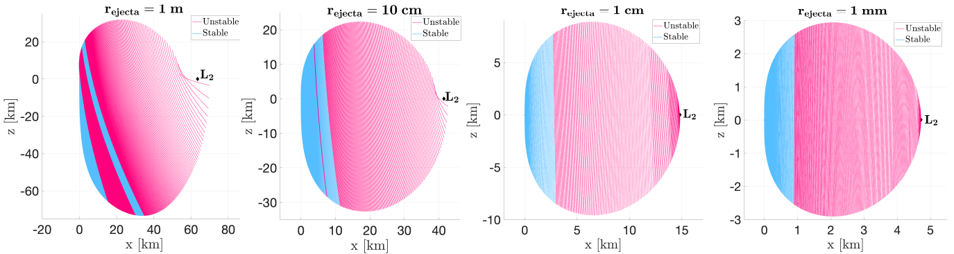
Figure 6. Terminator orbits originating from L_2 in the augmented CRTBP model for spherical ejecta with different radii. The combined mass of Didymos and Dimorphos is located at the origin of the secondary-centered synodic frame. From left to right, the subplots correspond to ejecta radii of 1 m, 10 cm, 1 cm, and 1 mm. Note that a smaller ejecta radius corresponds to a higher SRP acceleration of the ejecta.
