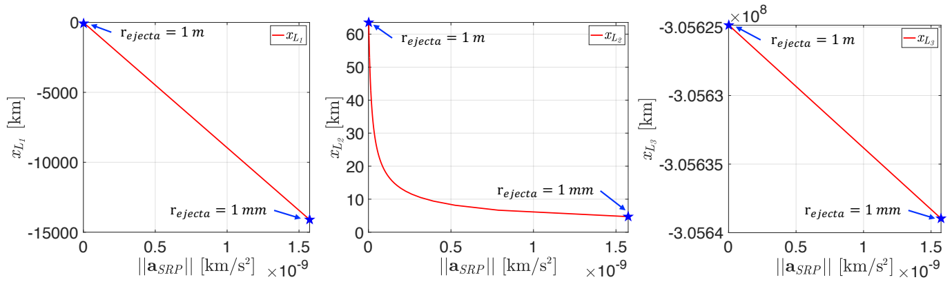
Figure 4. The variation of the x -coordinates of the collinear EPs in the augmented Sun–Didymos and Dimorphos system with respect to the SRP acceleration magnitude \|\mathbf{a}_{\text{SRP}}\| . The locations of EPs are represented in the synodic frame centered on the secondary, which coincides with the origin of this frame.
