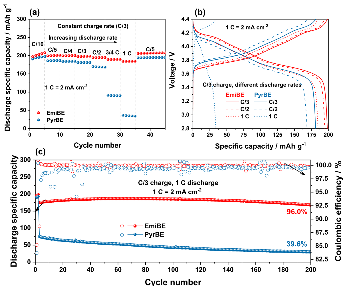
Fig. 5. Performance of Li/NMC811 cells employing EmiBE and PyrBE electrolytes. (a) Rate performance at different discharge C-rates with a constant charge rate of C/3 after five formation cycles at C/10. (b) The dis-/charge profiles of the cells at few selected C-rate. (c) The evolution of CE and discharge specific capacity upon long-term cycling of the cells with a charge rate of C/3 and a discharge rate of 1C after two formation cycles at C/10. The mass loading of NMC811 is 10 mg cm -2 . 1C is 200 mA g -1 , equaling to 2 mA cm -2 .
