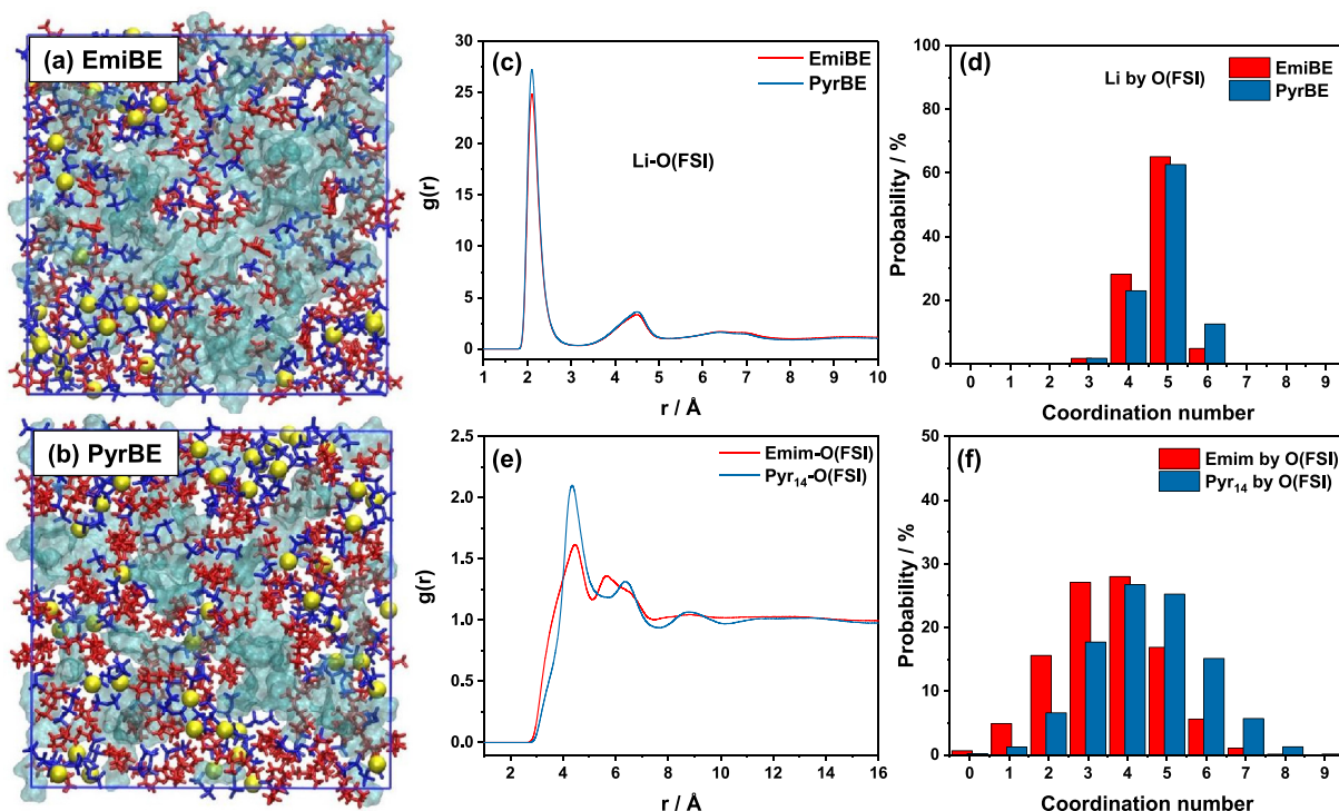
Fig. 2. MD simulation for the EmiBE and PyrBE electrolytes. Snapshots of the MD simulated boxes for (a) EmiBE and (b) PyrBE electrolytes. The yellow spheres, red sticks, blue sticks, and cyan clouds represent \text{Li}^+ , organic cation, \text{FSI}^- , and BTFE, respectively. Radial distribution functions of (c) Li-O(FSI) and (e) Emim/Pyr 14 -O(FSI) pairs. Coordination number populations of (d) Li by O(FSI), (e) Emim/Pyr 14 by O(FSI).
