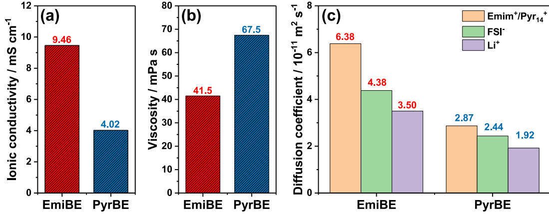
Fig. 1. (a) Ionic conductivities and (b) viscosities of EmiBE and PyrBE at 20 °C. (c) Self-diffusion coefficients of ions in EmiBE and PyrBE measured via PFG-NMR at 20 °C.
