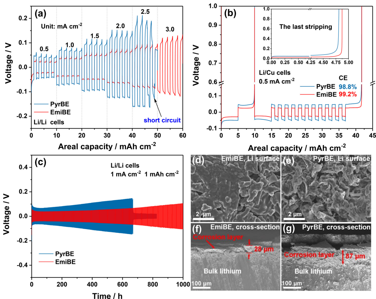
Fig. 3. (a) Voltage profiles of Li plating/stripping processes in Li/Li cells at various current densities. (b) Li plating/stripping CE in Li/Cu cells. The inset shows the voltage profile of the last stripping process. (c) Long-term cycling voltage profiles for Li/Li cells. (d,e) Surface and (f,g) cross-section morphology of the Li foil after 100 cycles with a current density of 1 \text{ mA cm}^{-2} and a stripping-plating areal capacity of 1 \text{ mA cm}^{-2} in (d,f) EmiBE and (e,g) PyrBE electrolytes.
