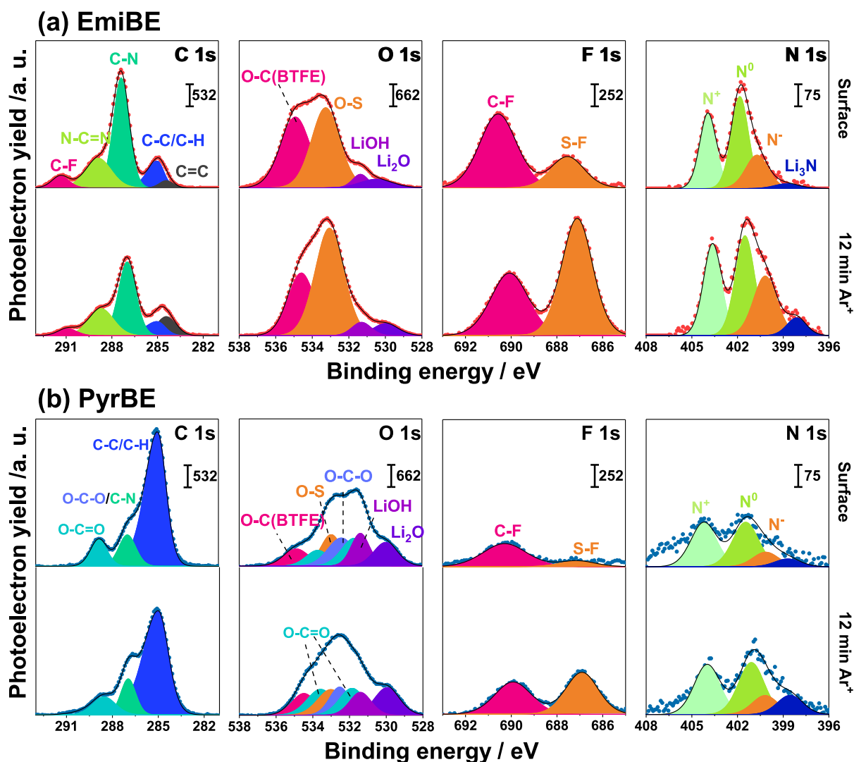
Fig. 4. XPS analysis of C 1s, O 1s, F 1s, and N 1s photoelectron lines for the lithium ( 1.5 \text{ mAh cm}^{-2} ) deposited on Cu foil at 0.5 \text{ mA cm}^{-2} in (a) EmiBE and (b) PyrBE electrolyte (surface and after \text{Ar}^+ sputtering for 12 min).
