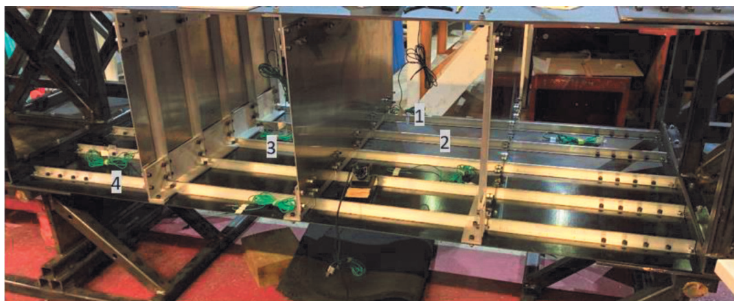
Fig. 13. Location of debonded stiffeners.
