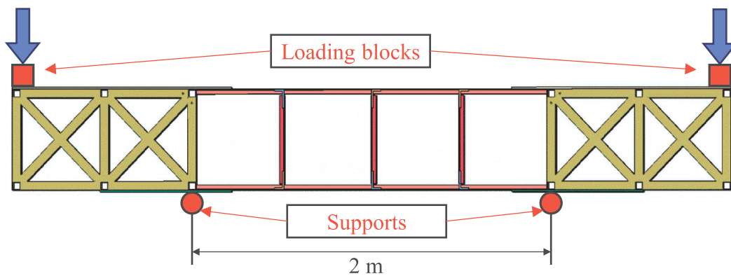
Fig. 5. 4-point bending configuration.
