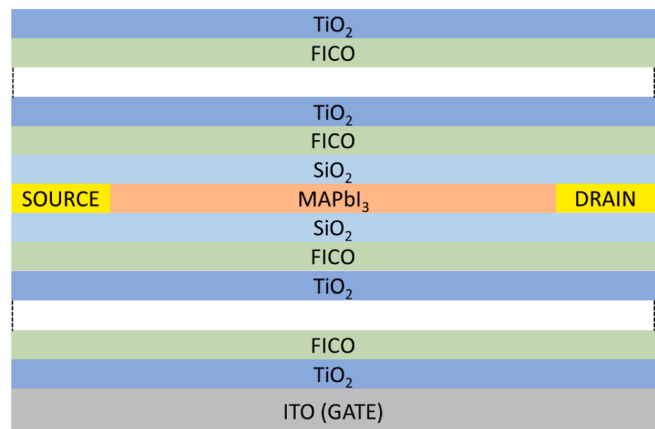
Fig. 1. Structure of the MaPbI 3 light-emitting field-effect transistor integrated with a microcavity composed by two FICO/TiO 2 one-dimensional photonic crystals with the MaPbI 3 layer as defect.
