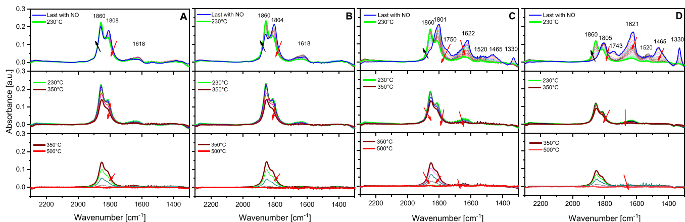
Fig. 11. - FT-IR spectra collected during the Temperature Programmed Desorption (TPD) after NO/O 2 adsorption at 150 °C (A), 120 °C (B), 80 °C (C), 60 °C (D). Experimental conditions: TPD in O 2 (3%) + CO 2 (2%) + H 2 O (1.5%) in He from 80 °C to 500 °C (10°/min).
