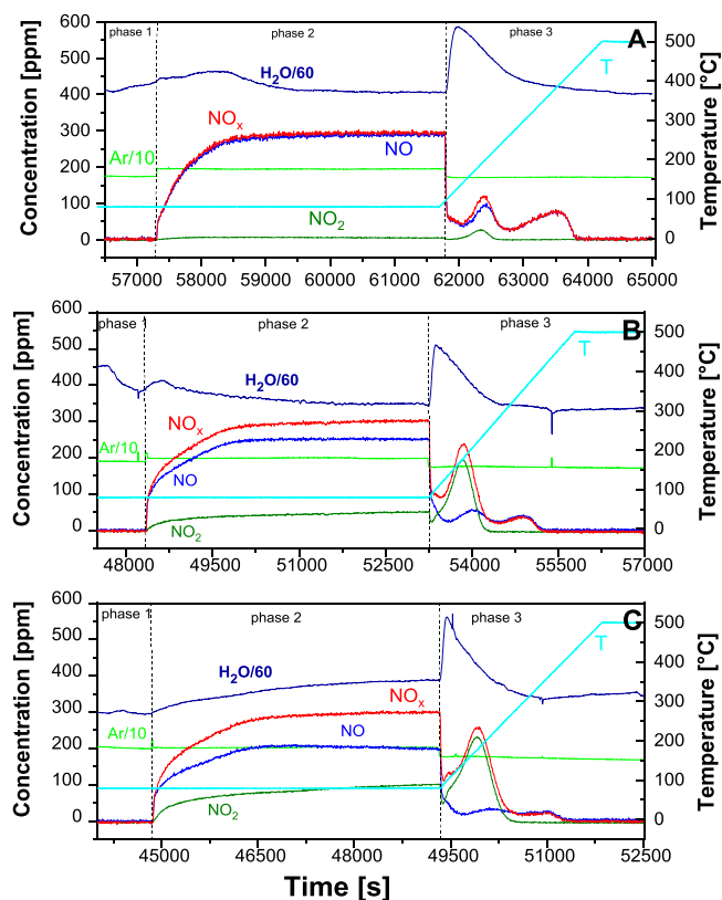
Fig. 13. - \text{NO}/\text{NO}_2/\text{O}_2 adsorption (phase 2) and subsequent TPD (phase 3) at 80 ^{\circ}\text{C} over \text{Pd}_1/\text{SSZ-13} . A) \text{NO}_2/\text{NO} ratio = 0; B) \text{NO}_2/\text{NO} ratio = 0.2; C) \text{NO}_2/\text{NO} ratio = 0.5. Experimental conditions: storage phase \text{NO} (300, 250 or 200 ppm) + \text{NO}_2 (0, 50 ppm or 100 ppm) + \text{O}_2 (3%) + \text{CO}_2 (2%) + \text{H}_2\text{O} (2.5%) in He. TPD in \text{O}_2 (3%) + \text{CO}_2 (2%) + \text{H}_2\text{O} (2.5%) in He from 80 ^{\circ}\text{C} to 500 ^{\circ}\text{C} (10 ^{\circ}/\text{min} ).
