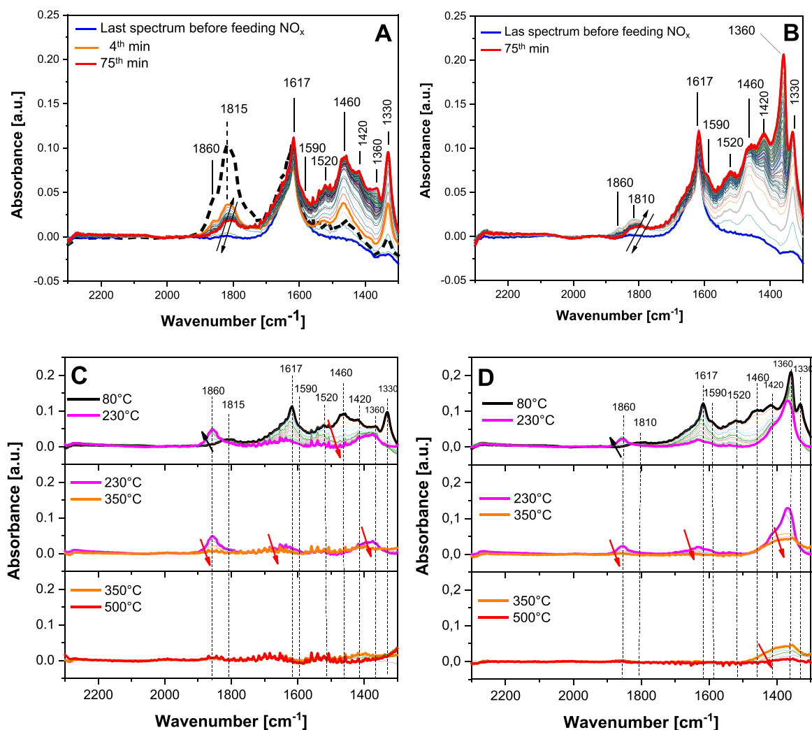
Fig. 14. - FT-IR spectra collected during the \text{NO}/\text{NO}_2/\text{O}_2 adsorption at 80 °C (A) \text{NO}_2 / \text{NO} ratio = 0.2; B) \text{NO}_2 / \text{NO} ratio = 0.5) and subsequent TPD (C and D, respectively). Experimental conditions: storage phase \text{NO} (250 or 200 ppm) + \text{NO}_2 (50 ppm or 100 ppm) + \text{O}_2 (3%) + \text{CO}_2 (2%) + \text{H}_2\text{O} (1.5%) in He. TPD in \text{O}_2 (3%) + \text{CO}_2 (2%) + \text{H}_2\text{O} (1.5%) in He from 80 °C to 500 °C (10°/min). Dotted spectrum reported in Fig. 14 A refers to \text{NO}/\text{O}_2 adsorption at 80 °C (i.e. without \text{NO}_2 ).
