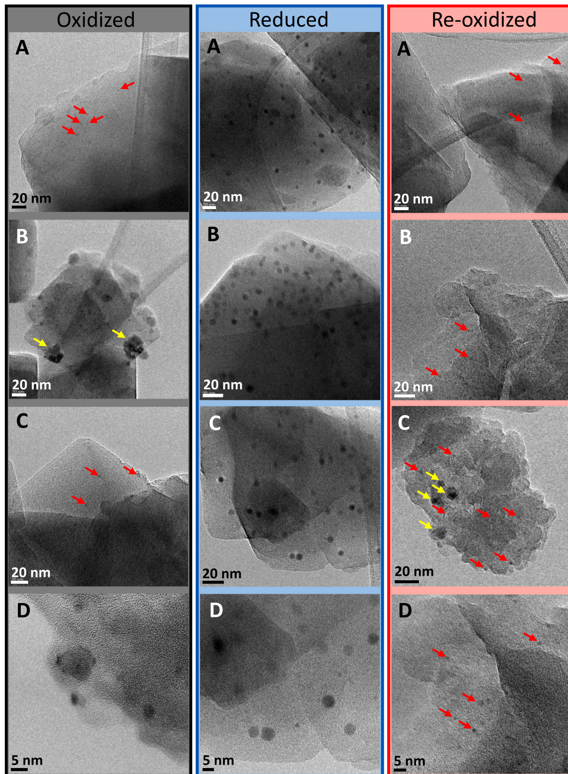
Fig. 1. - TEM and HR-TEM images of Pd 1 /SSZ-13 oxidized in O 2 (40 mbar) at 500 °C, reduced in H 2 (40 mbar) at 500 °C and re-oxidized in O 2 (40 mbar) at 500 °C. Red arrows: some less recognizable Pd particles; yellow arrows: Pd particle aggregates.
