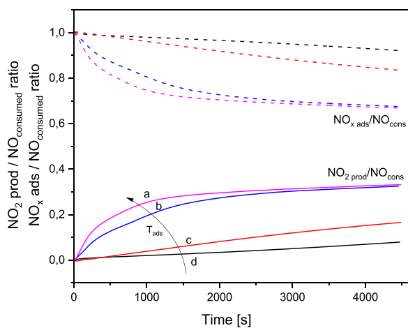
Fig. 10. - NO 2 produced in adsorption phase / NO consumed ratio (Solid lines); NO x adsorbed / NO consumed ratio (Dash lines): 150 °C (a), 120 °C (b), 80 °C (c), 50 (d).
