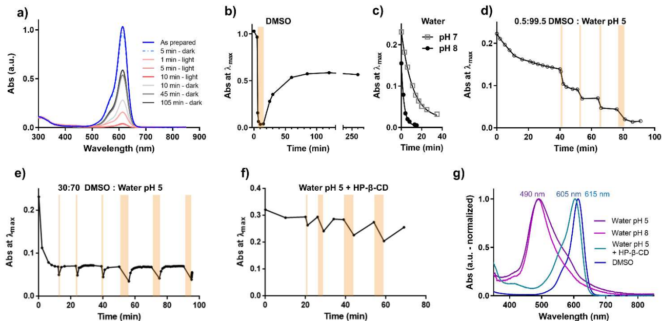
Figure 2. Reversible photoswitching of DASA-barbital in organic and aqueous media. a) UV/vis absorption spectra of 50 \mu M DASA-barbital in DMSO as prepared, after illumination with a halogen lamp (orange bars), and after thermal relaxation in the dark. b) Time course of 50 \mu M DASA-barbital absorption at peak (615 nm) in DMSO under illumination (orange bar, 10 min) and relaxation in the dark at room temperature. c) Spontaneous, irreversible conversion of 50 \mu M DASA-barbital in water at pH 8 (0.5% DMSO) and at pH 7 (1% DMSO). d) Photo-induced irreversible conversion is possible with 50 \mu M DASA-barbital in 0.5% DMSO:water at pH 5. Time course at absorption peak (490 nm) with illumination time of 1, 2, 3 and 10 minutes. e) Time course of 50 \mu M DASA-barbital during photoswitching cycles (1 or 5 min) in 30:70 DMSO:water at pH 5 at absorption peak (590 nm). f) Reversible photoswitching of 500 \mu M DASA-barbital in water at pH 5 can be achieved with 10% w/v HP- \beta -CD. Time course at absorption peak (605 nm) with illumination time of 1, 3 and 5 minutes. g) Normalized UV/vis absorption spectra of different solutions of DASA-barbital: water pH 5 (dark purple), water pH 8 (pink), DMSO (blue), and water and HP- \beta -CD 10% w/v pH 5 (light blue). DASA-barbital is thus exposed to a hydrophobic environment in HP- \beta -CD.
