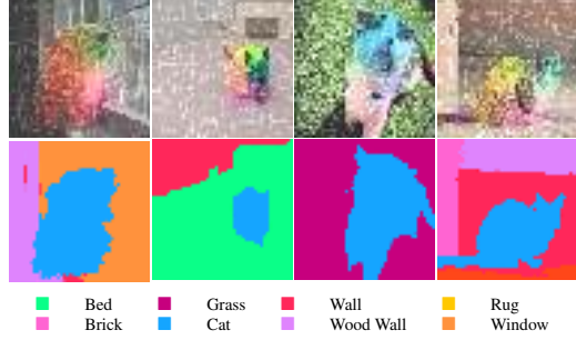
Figure 3: \partial HT tokenized images with feature correspondences (top) and semantic segmentation (bottom).
