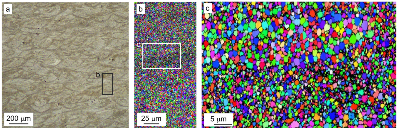
Figure 3. Microstructure of the vertical section of as-built sample after chemical etching with Keller's reagent (a). LOM image and EBSD orientation maps (b) including (c) in the area straddling two laser tracks.
