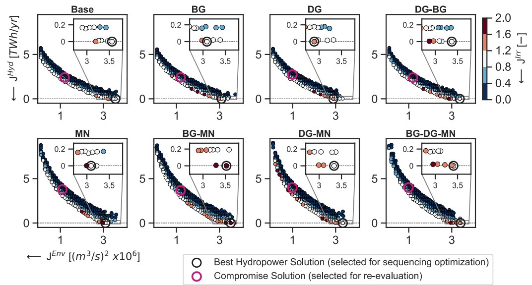
Figure 3. Pareto reference sets of operating policies for the existing (Base) and seven candidate reservoir network configurations which include one or more of the three planned reservoirs (reservoir key: Batoka Gorge (BG); Devils Gorge (DG); Mphanda Nkuwa (MN)). To facilitate cross-comparison of the reference sets, the hydropower deficit ( J^{Hyd} ) is plotted relative to the minimum deficit achieved under a given reservoir network configuration. The “best hydropower” solution selected for the sequencing optimization is indicated with an open black circle on the main and inset plot. The “compromise” solution (closest to ideal point in normalized objective space) is identified with an open pink circle.
