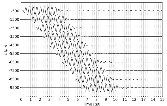
Fig. 23 Test case of Sect. 6.3. The figure shows the acoustic pressure computed at ten equispaced points P = (0, 0, z) , with z \in \{-500 \mu\text{m}, \dots, -9500 \mu\text{m}\}
