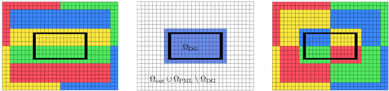
Fig. 5 Schematic illustration of the outer domain decomposition: non-optimized partitioning (left), DG layer \Omega_{DG} (middle), optimal partitioning (right). The set of processors is \{P_1, P_2, P_3, P_4\} = \{\text{blue}, \text{yellow}, \text{red}, \text{green}\} . (color figure online)
