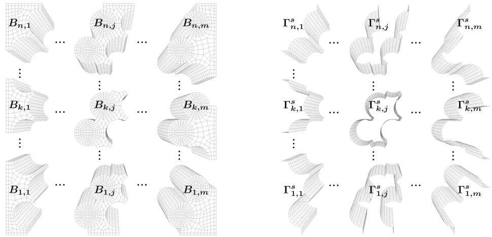
Fig. 7 Schematic representation of the mesh partitioning into blocks B_{n,m} (left) and the corresponding interfaces \Gamma_{n,m}^s , with n = 1, \dots, N_{\text{block}} and m = 1, \dots, M , used for block merging (right). The blocks illustrate the content of the elementary files f_s^{\text{el}} owned by the computational processes. Repetition of these blocks along the x - and y -directions allows the computational domain to be extended to an arbitrary size
