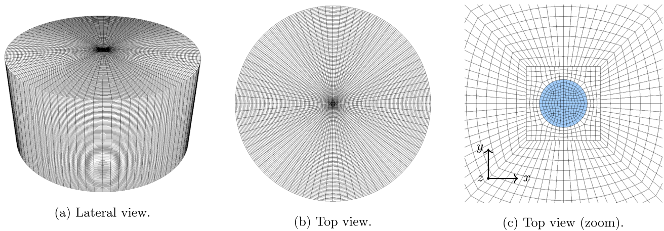
Fig. 10 Test case of Sect. 6.1. Mesh configuration used for the single PMUT simulation. Panels a–c show the lateral, top, and zoomed top views, respectively. The PMUT, highlighted in panel (c), is excited by an input voltage signal applied to its upper surface
