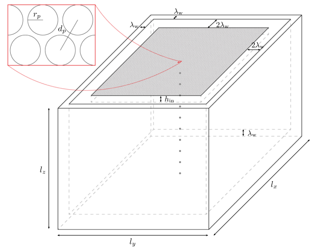
Fig. 21 Test case of Sect. 6.3. Representation of the three-dimensional view of the geometry employed for the 64-elements simulation. The dots represent the probes at which the solution is computed. Notice that the figure is not scaled
