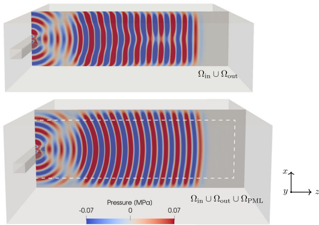
Fig. 19 Test case of Sect. 6.3. Schematic representation of a slice of the acoustic domain \Omega_{\text{in}} \cup \Omega_{\text{out}} and the surrounding perfectly matched layer region \Omega_{\text{PML}} . The upper figure corresponds to the simulation without the PML, while the lower figure shows the solution obtained when the PML is included. The dashed line represents the interface \Gamma_{\text{PML}}
