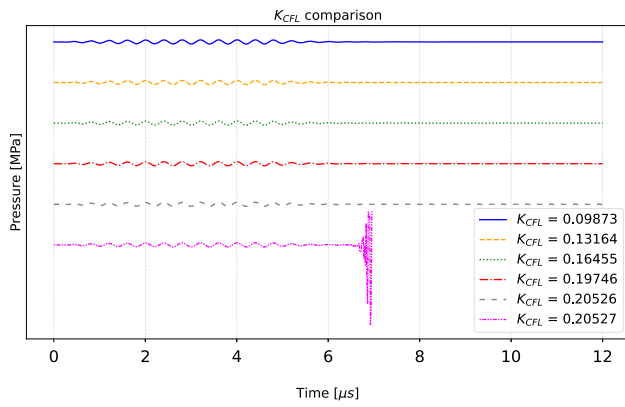
Fig. 14 Test case of Sect. 6.1. Stability analysis under varying K_{CFL} . The simulation remains stable up to the optimal value K_{CFL} = 0.20526 (grey curve), while a marginal increase to K_{CFL} = 0.20527 (magenta curve) triggers exponential numerical instability near the end of the simulation timeline. Curves are vertically offset for visual clarity
