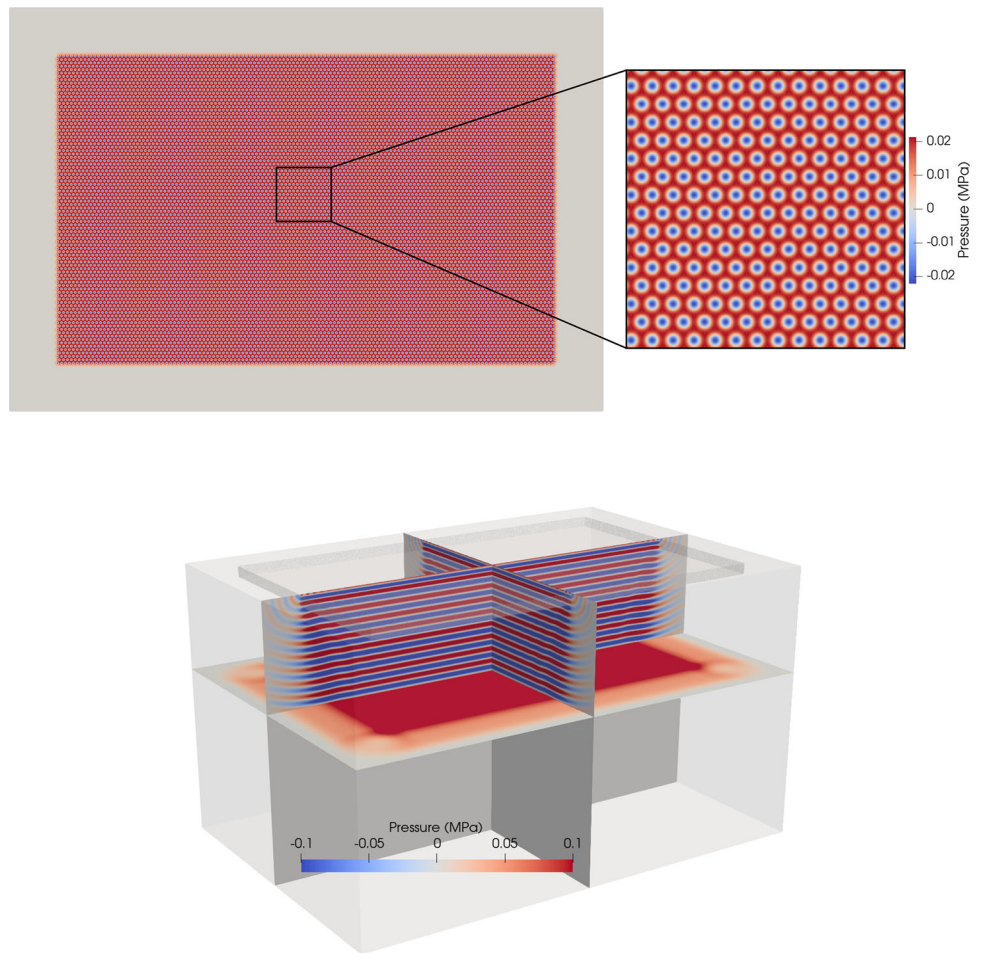
Fig. 22 Test case of Sect. 6.3. The figure shows the snapshot of the surface containing the PMUTs at time t = 0.2 \mu\text{s} with a zoom of the middle region (top), and the solution at time t = 4 \mu\text{s} depicted over 3 slices (bottom)
