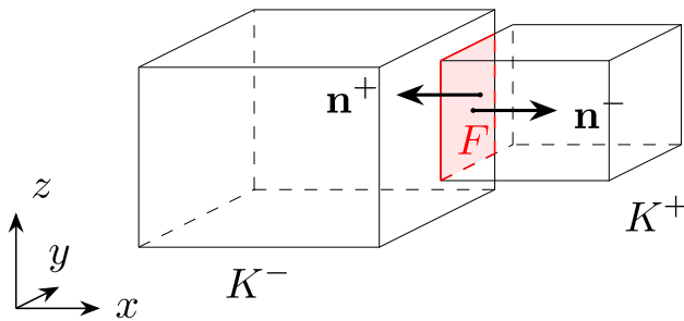
Fig. 4 Representation of two adjacent hexahedra K^+ and K^- with the shared face F and the corresponding normal vectors \mathbf{n}^+ and \mathbf{n}^-
