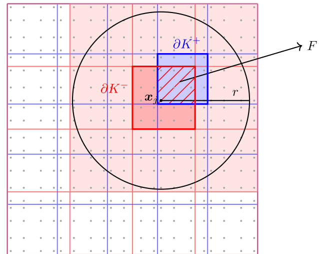
Fig. 9 Example of the matching algorithm of DG faces. The red and blue grids refer to the coarse and fine faces, respectively, and the grey dots are the Gauss-Legendre quadrature nodes of the finer faces. The blue-filled face is a representative fine face, and the center \mathbf{x}_j of the circle is its quadrature node considered; the red-filled faces are those selected by the algorithm. Notice that considering only one vertex of the coarse face instead of all four increases the number of residual faces, but it avoids excessive RAM consumption. (color figure online)
