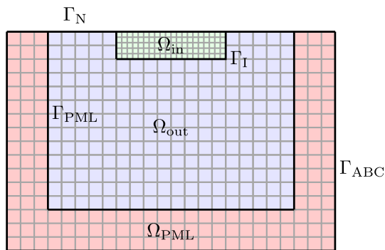
Fig. 3 Example of mesh employed in the DG-SE approach. Different mesh sizes and polynomial degrees are employed for \Omega_{in} and \Omega_{out} , resulting in a non-conforming mesh
