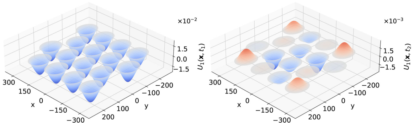
Fig. 20 Test case of Sect. 6.3. Three-dimensional surface plots showing the spatial evolution of the array-centered PMUTs displacement field U_k(\mathbf{x}, t) in \mu\text{m} at two time instants: t_1 = 0.4 \mu\text{s} , t_2 = 10.4 \mu\text{s}
