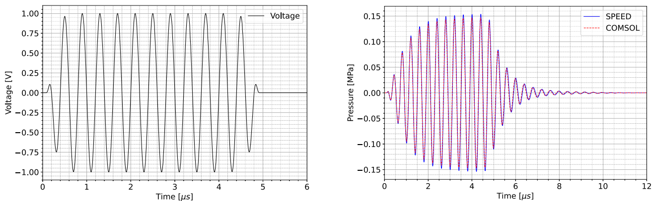
Fig. 11 Test case of Sect. 6.1. Time evolution of the input signal imposed on the PMUT surface (left), and output pressure computed at the PMUT center (right). SPEED and COMSOL signals are in blue and red, respectively. (color figure online)
