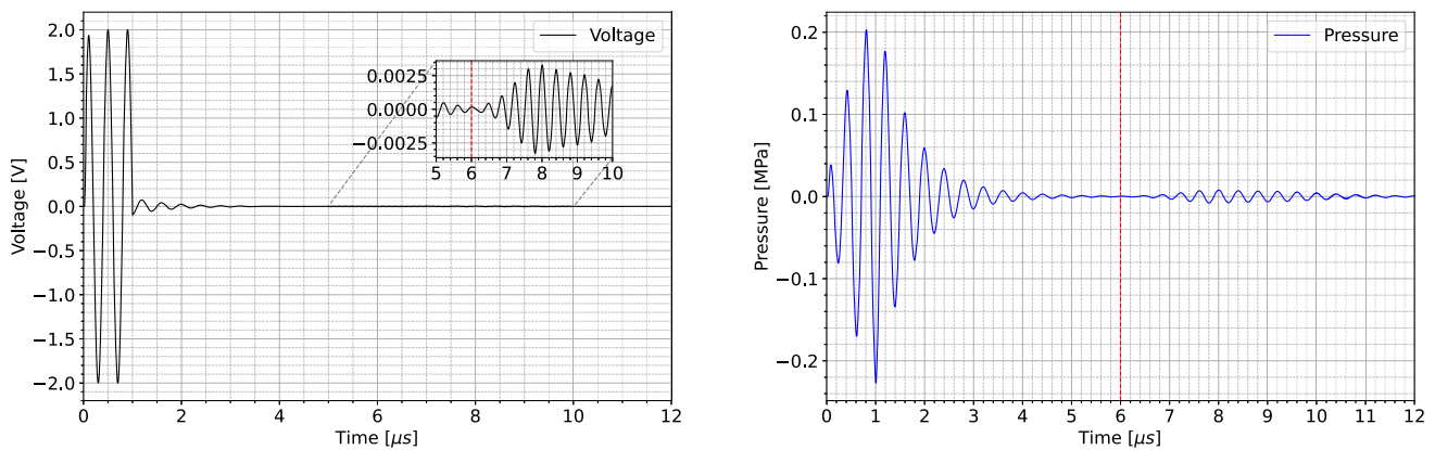
Fig. 16 Test case of Sect. 6.2. Time evolution of the input signal imposed on the PMUT surface (left) with a zoom on the region for t \in [5, 10] \mu\text{s} , and output pressure computed at the PMUT center (right). The time instant t = 6T_d is highlighted with a dashed line
