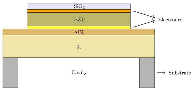
Fig. 1 Cross-section of a representative PMUT stack, illustrating the multilayer structure in which each layer has a defined thickness and distinct material properties
