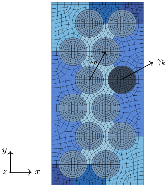
Fig. 6 Top view of a minimal example of inner domain \Omega_{in} . The elementary structures originating \Omega_{in} are depicted with different colors. The circular regions represent the membranes \gamma_k belonging to \Gamma_{PMUT} , while the remaining part is \Gamma_N . (color figure online)
