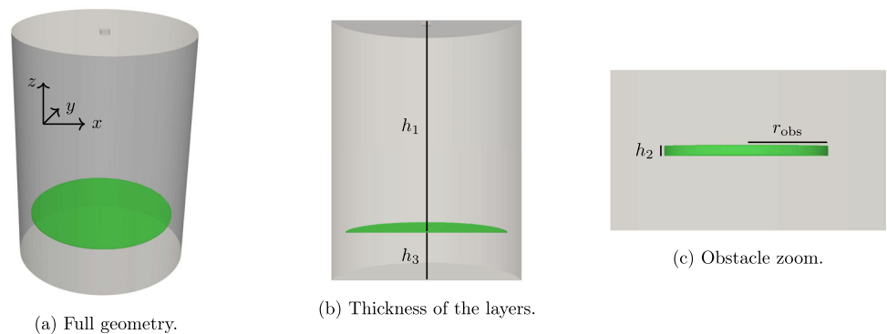
Fig. 15 Test case of Sect. 6.2. Geometry used for the single PMUT simulation with an obstacle in TX-RX phases. Panels a–c show the geometry employed, the thickness of the cylinder layers, and a zoom of a representative obstacle for graphical reasons, respectively
