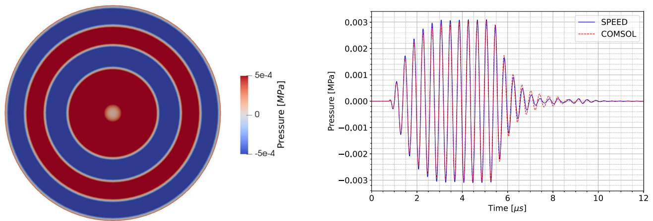
Fig. 12 Test case of Sect. 6.1. Snapshot at t = 4 \mu\text{s} of a slice in the x - y plane (left), and output pressure computed at the P = (0 \mu\text{m}, 0 \mu\text{m}, -1000 \mu\text{m}) for SPEED and COMSOL (right)
