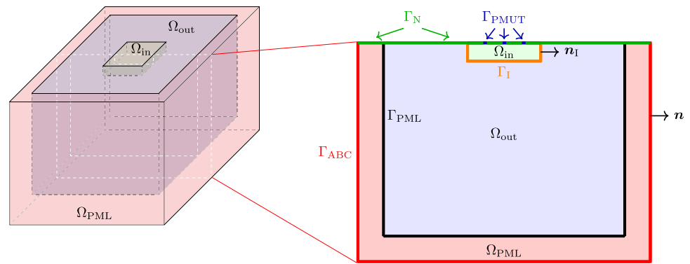
Fig. 2 A three-dimensional view of the domain decomposition (left) and the corresponding two-dimensional slice with boundary labels (right) for problem (1). For the sake of completeness, in these pictures, we consider the presence of \Omega_{\text{PML}} . When \Omega_{\text{PML}} = \emptyset , then \Gamma_{\text{PML}} reduces to \Gamma_{\text{ABC}}
