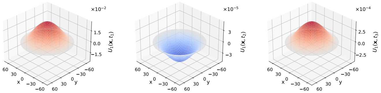
Fig. 18 Test case of Sect. 6.2. Three-dimensional surface plots showing the time evolution of the PMUT membrane displacement field U_1(\mathbf{x}, t) in \mu\text{m} for the TX-RX configuration at three time instants: t_1 = 1.0 \mu\text{s} , t_2 = 6.0 \mu\text{s} , t_3 = 10.2 \mu\text{s}
