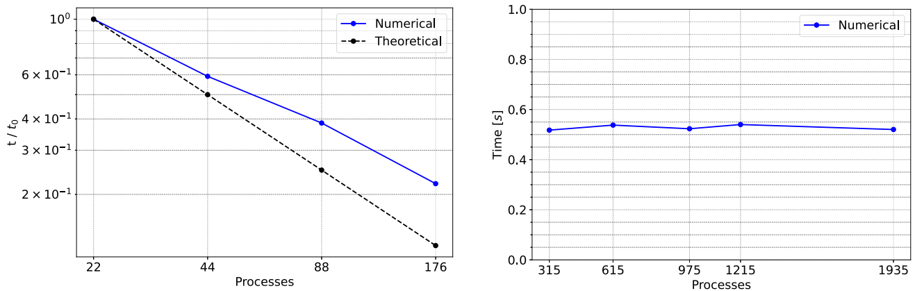
Fig. 24 Test case of Sect. 6.4. The figure shows the theoretical trend (black) and the real one (blue) of the strong scalability test conducted across four different simulations (left). The value on the y-axis is nor-
