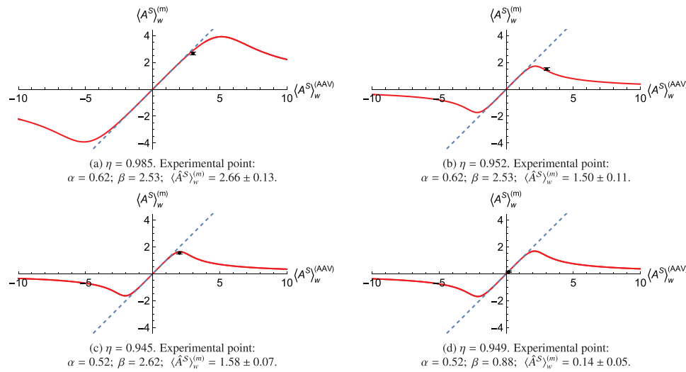
Figure 2. Discrepancy between \langle \hat{A}^S_w \rangle_w^{(m)} expected from a N = 7 steps RWM protocol and the one corresponding to the full pre- and postselection case ( \eta \rightarrow 1 ) \langle \hat{A}^S_w \rangle_w^{(AAV)} = \langle \psi_\beta | \hat{A}^S | \psi_\alpha \rangle / \langle \psi_\beta | \psi_\alpha \rangle , for four different \eta values and pre- and postselection angles \alpha and \beta . The dashed blue line represents the condition \langle \hat{A}^S_w \rangle_w^{(m)} = \langle \hat{A}^S_w \rangle_w^{(AAV)} , while the red continuous curve shows the RWM outcome behavior for \eta \lesssim 1 . The black dots and bars represent, respectively, the experimental results and associated uncertainties obtained with our RWM procedure in ref. [73].
