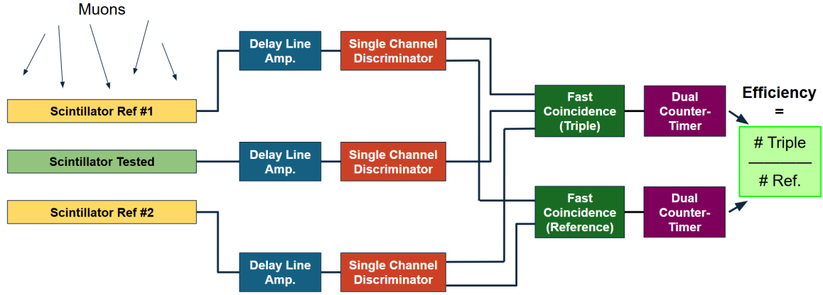
Figure 14. Scintillator efficiencies measurement setup.
