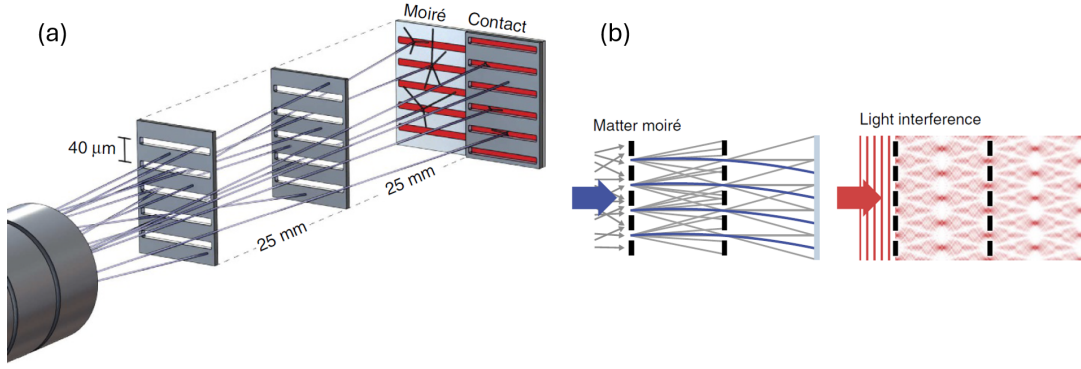
Figure 1. (a,b) Deflectometer functioning principle, where antihydrogen atoms pass through two gratings and form a fringe pattern. Reproduced from [5]. CC BY 4.0.
