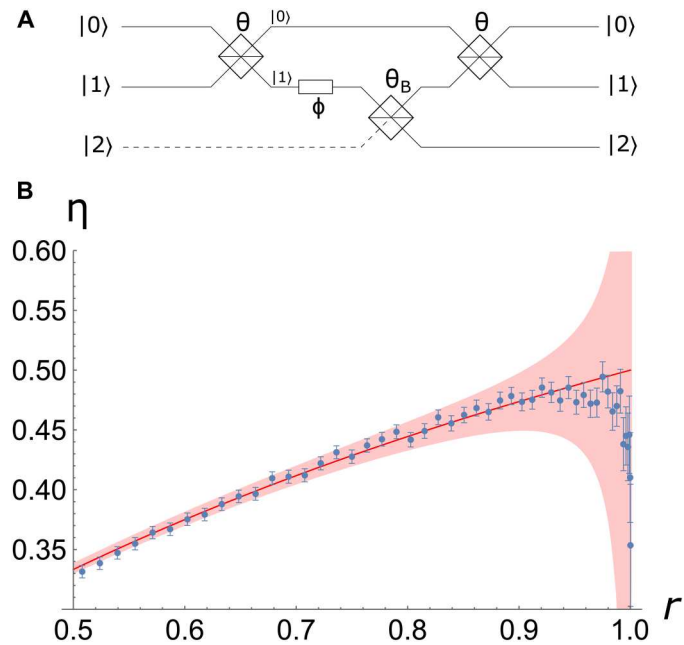
Fig. 3. Coherence and contextuality in a MZI. (A) Scheme of the circuit used for the quantum interrogation task. (B) Efficiency \eta of the object’s detection versus the reflectivity r = \sin\theta of the two beam splitters in the MZI. The red curve is the theoretical prediction, while the red shaded area represents the deviations from the ideal model due to dark counts and imperfect calibration of the beam splitters. The error bars derive from the poissonian statistics of the single-photon counts.
