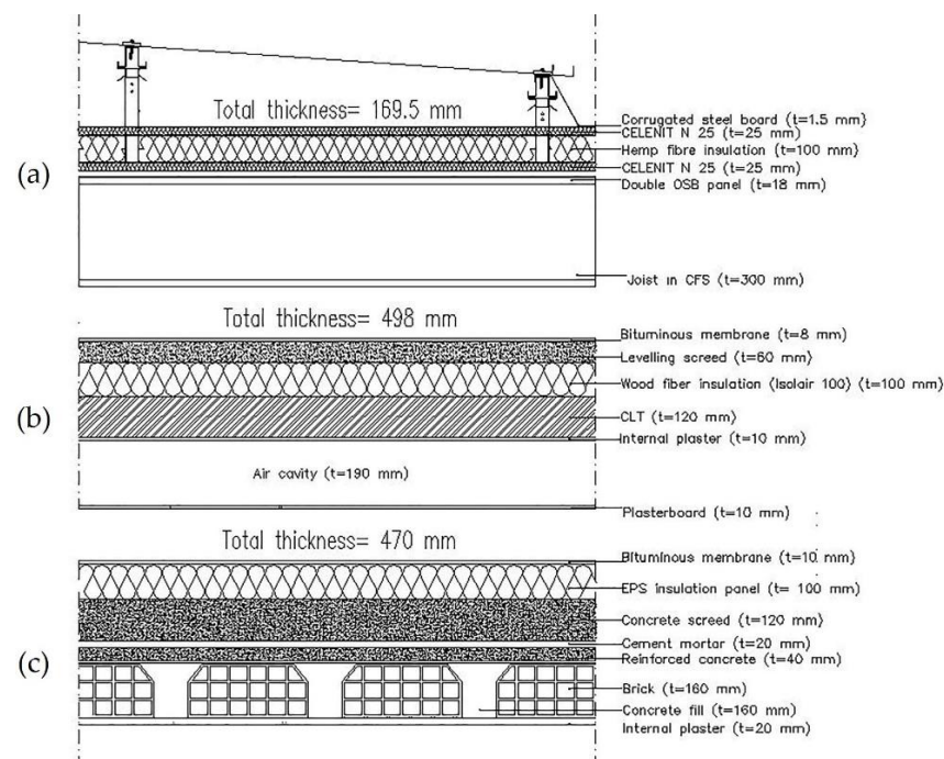
Figure 9. Roof configurations: (a) CFS; (b) CLT; (c) traditional.
