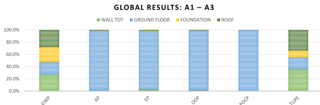
Figure 10. LCIA results: incidence percentages in each impact category.
