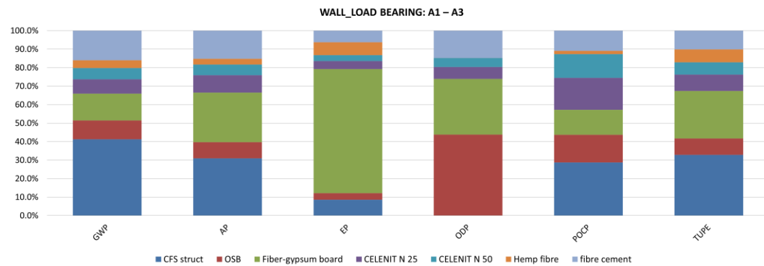
Figure 11. LCIA results: load-bearing walls.
