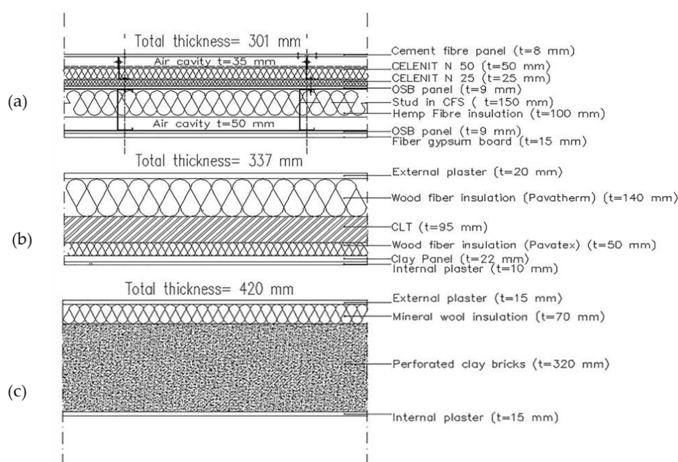
Figure 8. Wall configurations: (a) CFS; (b) CLT; (c) traditional.
