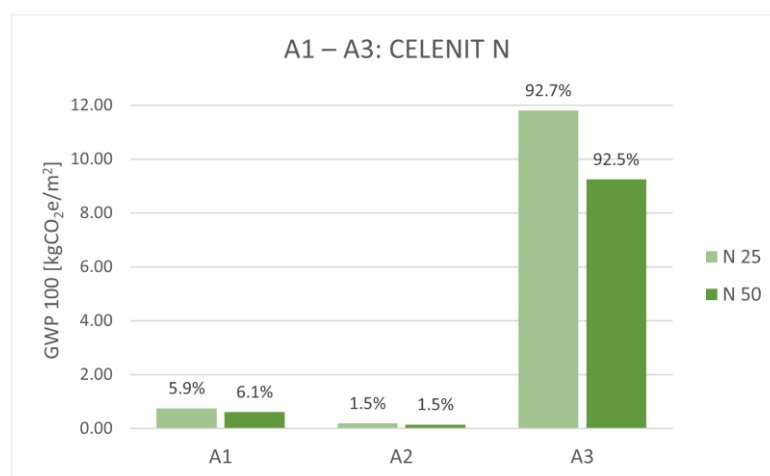
Figure 14. LCIA results for CELENIT N (25 mm and 50 mm).
