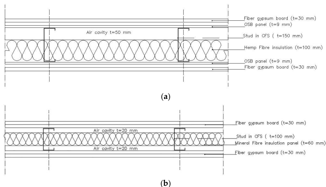
Figure 4. Internal wall sections: (a) load-bearing wall; (b) non-load-bearing wall.
