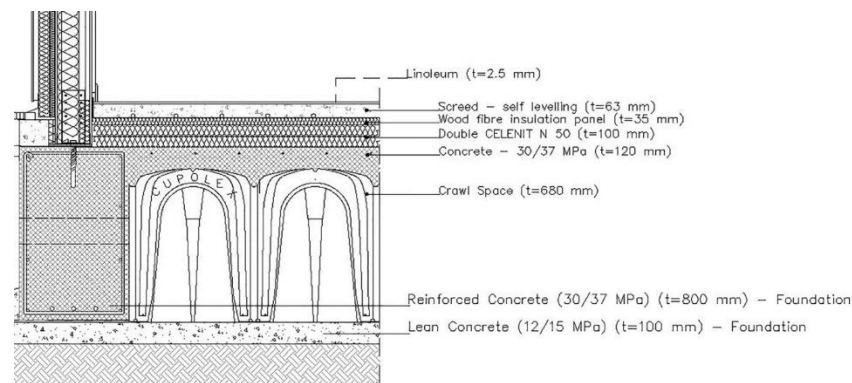
Figure 2. Foundation and ground floor sections.
