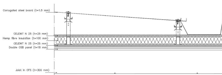
Figure 5. Roof section.
