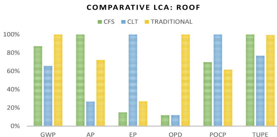
Figure 16. Results of Life Cycle impact assessment: Roof.
