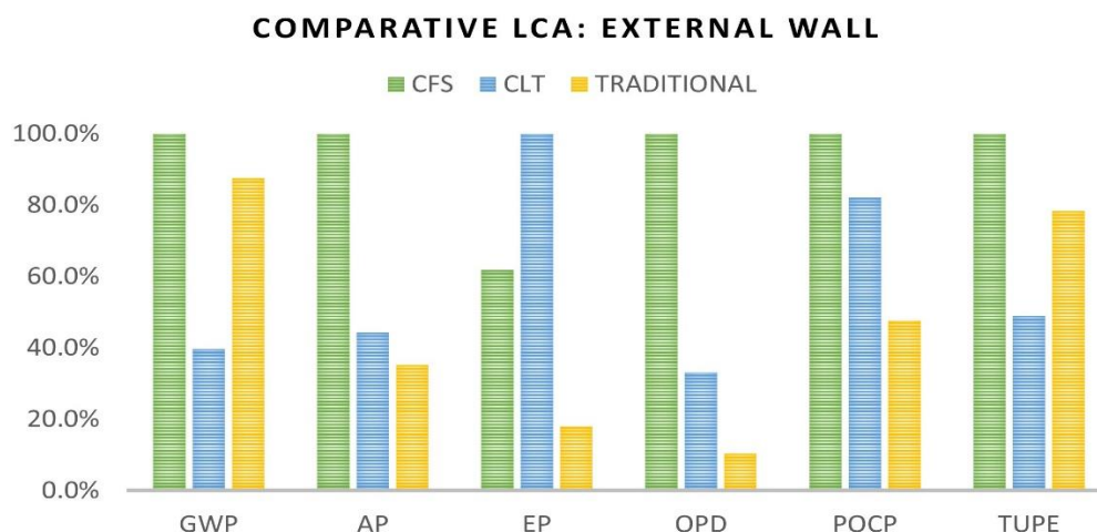
Figure 15. Results of Life Cycle impact assessment: External Wall.
