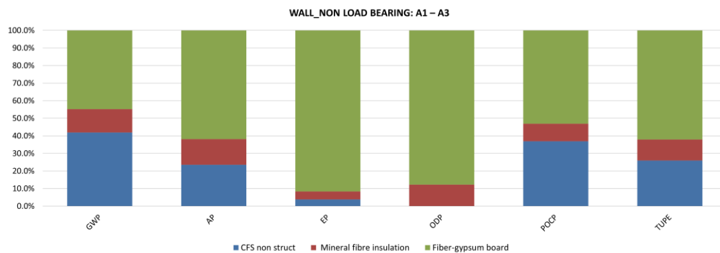
Figure 12. LCIA results: non-load-bearing walls.
