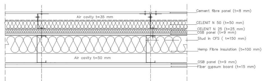
Figure 3. External wall section of the British Foundation school.
