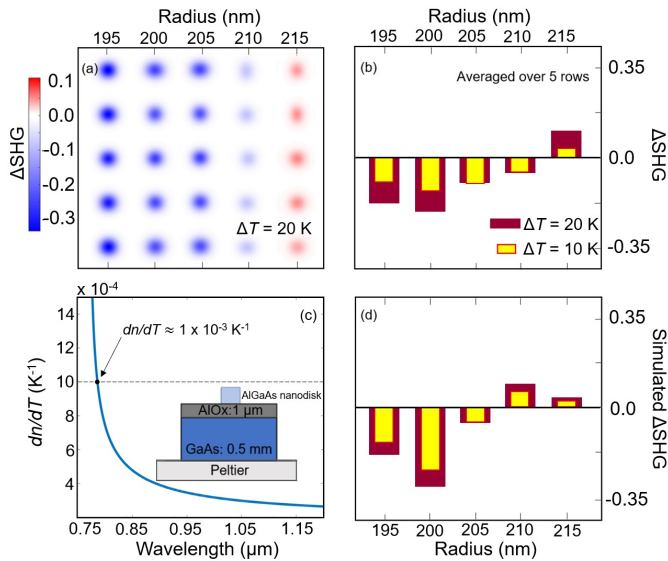
Fig. 2. (a) \Delta SHG(T_0 + 20\text{ K}) measured on five replicas (from top to bottom) of five different nanopillars. The average of \Delta SHG(T_0 + \Delta T) over each column in panel (a) is reported as red and yellow histograms in panel (b), for the five different radii and two different temperatures ( \Delta T = 10\text{ K} and \Delta T = 20\text{ K} ) (c) Theoretical model of dn/dT versus wavelength. Inset: schematic of the Peltier cell heating. (d) Modeling data to be compared with the experimental data reported in panel (b).
