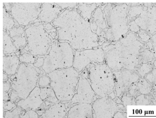
Fig. 3. Microstructure of the studied steel before hot deformation.
