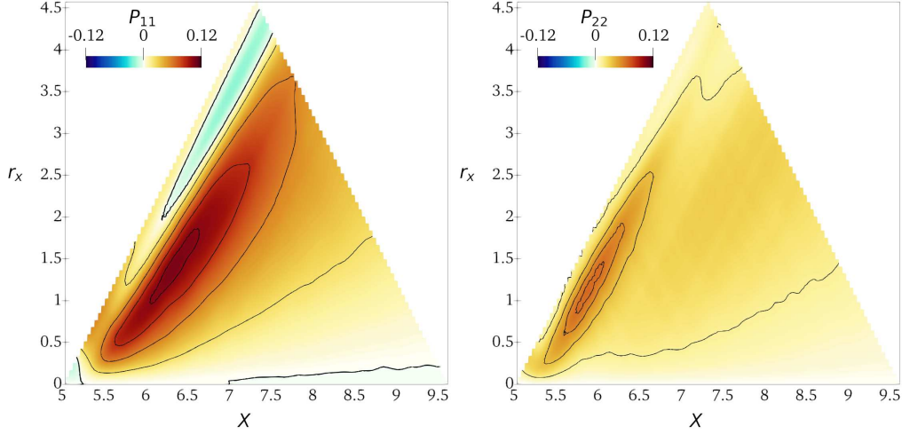
FIGURE 22. Production terms in the (X, r_x) space, r_y = r_z = 0 and Y = 0.38 .
