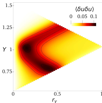
FIGURE 7. \langle \delta u \delta u \rangle in the (Y, r_y) space with r_x = r_z = 0 , X = 1.5 and 0.5 \leq Y \leq 1.55 .
