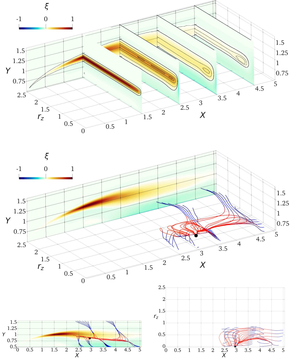
FIGURE 14. Field lines of the reduced fluxes for \langle \delta q^2 \rangle in the r_x = r_y = 0 space. The top panel is for the source term \xi . In the central panel the colourmap on the r_z = 2.5 plane is for \xi and the lines are coloured with the divergence of the reduced flux vector \nabla \cdot \hat{\Phi} : red/blue indicates positive/negative \nabla \cdot \hat{\Phi} . The lower panels are bottom and side views of the central one.
