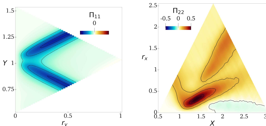
FIGURE 11. As figure 9, but for the pressure strain terms.
