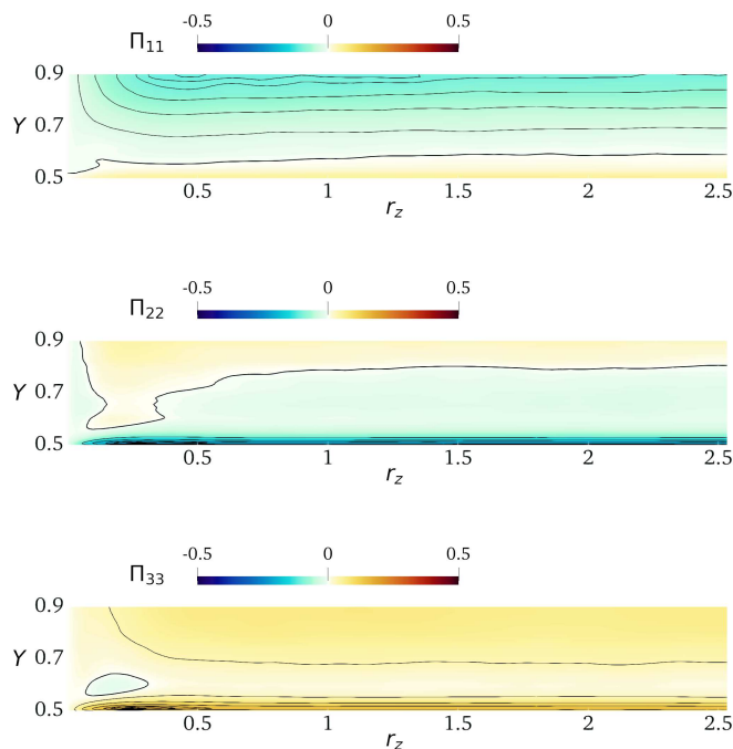
FIGURE 12. Two-dimensional view of the pressure-strain terms, in the plane X = 4 . Panels as in figure 10.
