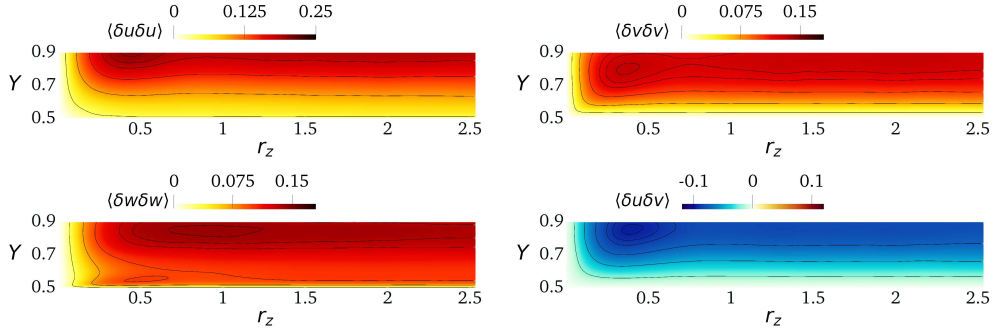
FIGURE 5. Two-dimensional view of the structure functions terms, in the plane X = 3.5 . Panels as in figure 4.
