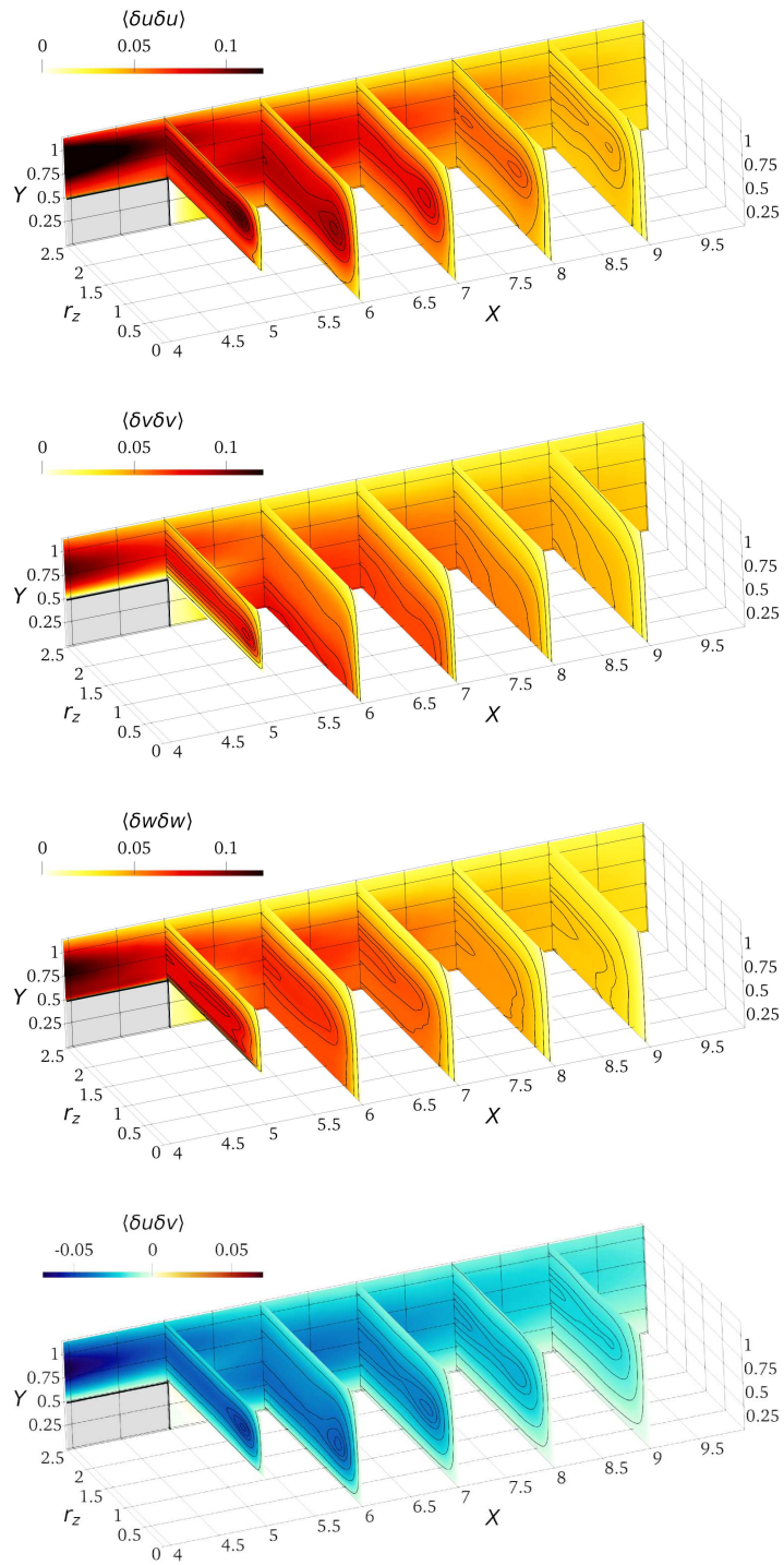
FIGURE 17. Components of the structure function tensor plotted in the space (X, Y, r_z) in the near wake.
