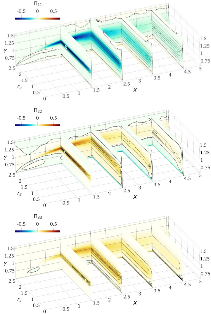
FIGURE 10. Top: \Pi_{11} ; centre: \Pi_{22} ; bottom: \Pi_{33} . The thick black line marks the zero contour level. White crosses are used to identify local maxima when not easily visible.
