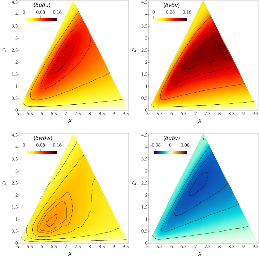
FIGURE 20. (X, r_x) space with r_y = r_z = 0 , Y = 0.38 and 5 \leq X \leq 9.5 .
