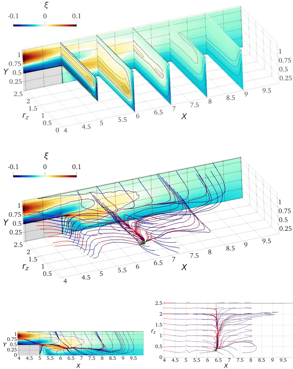
FIGURE 24. As figure 14, but for the near-wake region 4 \leq X \leq 10 and 0 \leq Y \leq 1 .
