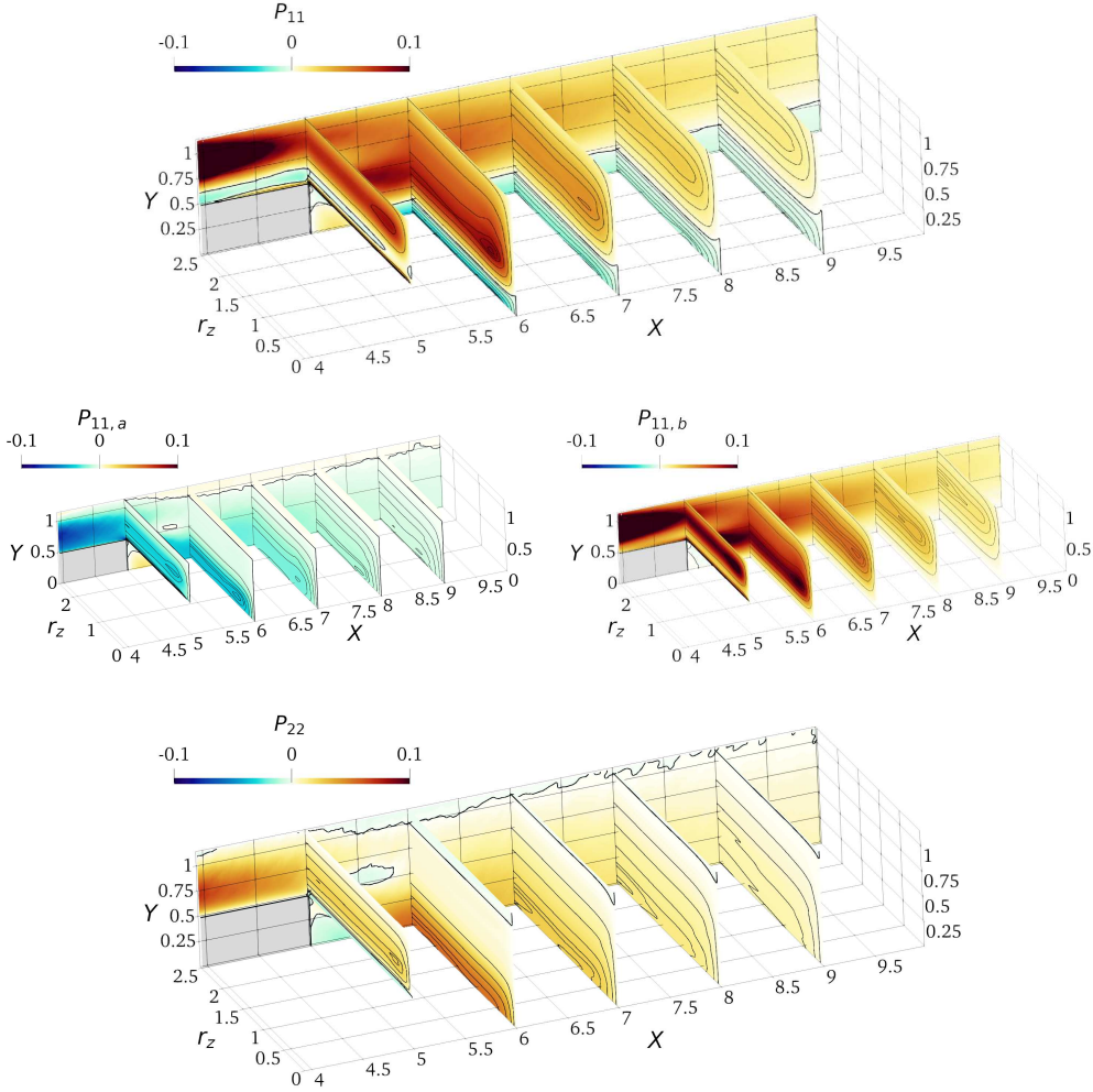
FIGURE 18. As in figure 8, but for 4 \leq X \leq 10 and 0 \leq Y \leq 1.1 .
