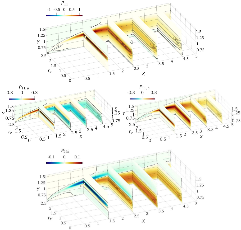
FIGURE 8. Top: P_{11} (with the two contributions P_{11,a} and P_{11,b} plotted separately in the central row). Bottom: P_{22,b} . The thick black line marks the zero contour level. White crosses are used to identify local maxima when not easily visible.
