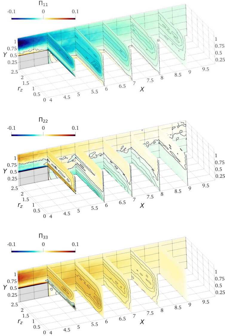
FIGURE 19. As figure 10, but for 4 \leq X \leq 10 and 0 \leq Y \leq 1.1 .
