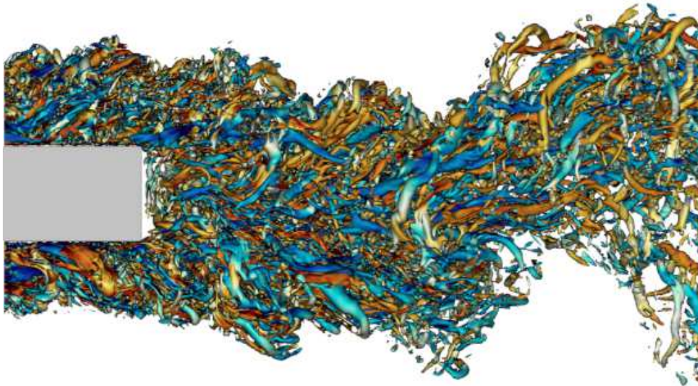
FIGURE 15. Instantaneous snapshot of the BARC flow: lateral view of the isosurfaces at \lambda_2 = -5 , with zoom into the near-wake region. Colour depicts streamwise vorticity \omega_x , with the blue-to-red colormap ranging in -10 \leq \omega_x \leq 10 . The vertical size D of the cylinder can be used as reference to identify the vertical and streamwise length scales of the near wake.
