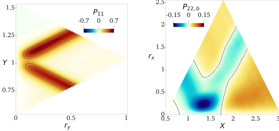
FIGURE 9. Production terms for \langle \delta u \delta u \rangle and \langle \delta v \delta v \rangle associated with the KH rolls. Left: P_{11} in the (Y, r_y) space with r_x = r_z = 0 , X = 1.5 and 0.5 \leq Y \leq 1.55 . Right: P_{22} in the (X, r_x) space with r_y = r_z = 0 , Y = 0.99 and 0.5 \leq X \leq 3 .
