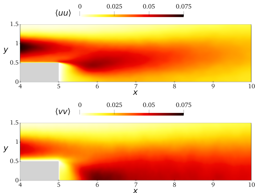
FIGURE 16. Maps of the \langle uu \rangle (top) and \langle vv \rangle (bottom) components of the Reynolds stresses in the x - y plane, with focus on the near wake.
