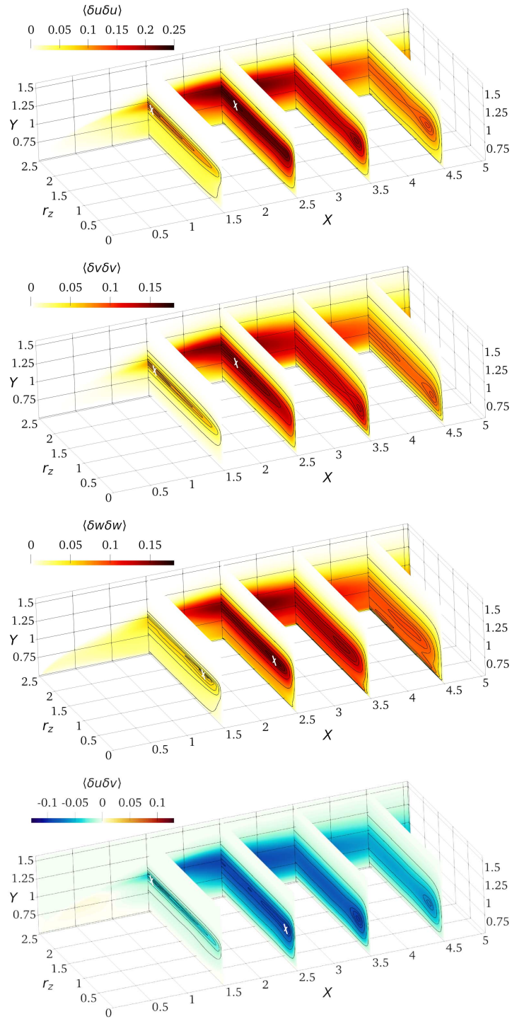
FIGURE 4. Components of the structure function tensor plotted in the space (X, Y, r_z) over the cylinder side. Contours in the planes X = 1.5, 2.5, 3.5, 4.5 are for the 99%, 95%, 90%, 75%, 50% and 20% of the in-plane maximum. White crosses are used to identify local maxima when not easily visible.
