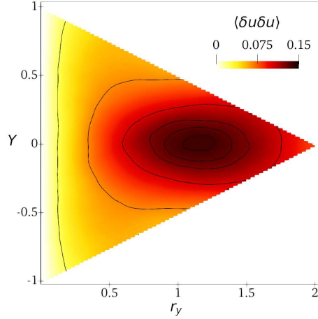
FIGURE 21. \langle \delta u \delta u \rangle in the (Y, r_y) space with r_x = r_z = 0 , X = 6.5 and -1 \leq Y \leq 1 .
