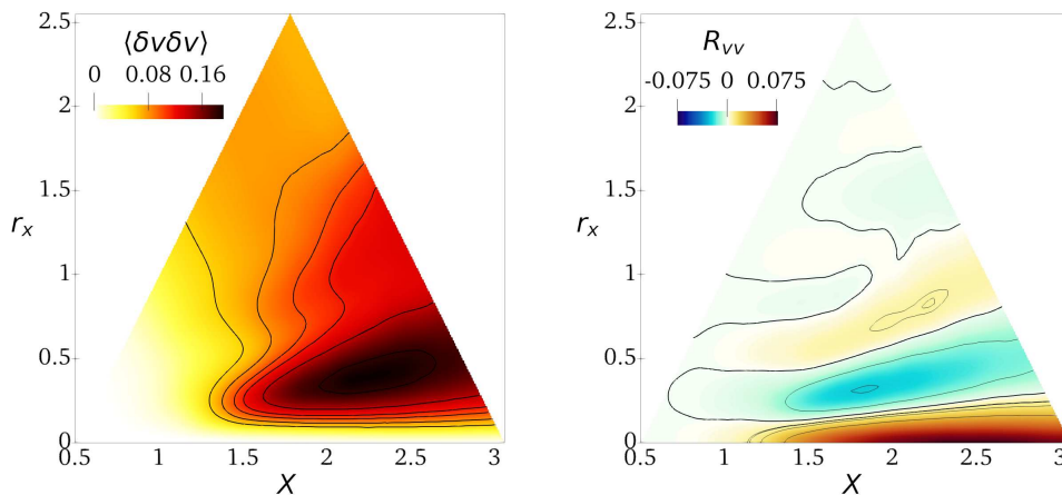
FIGURE 6. \langle \delta v \delta v \rangle (left) and R_{vv} (right) in the (X, r_x) space with r_y = r_z = 0 , Y = 0.99 and 0.5 \leq X \leq 3 .
