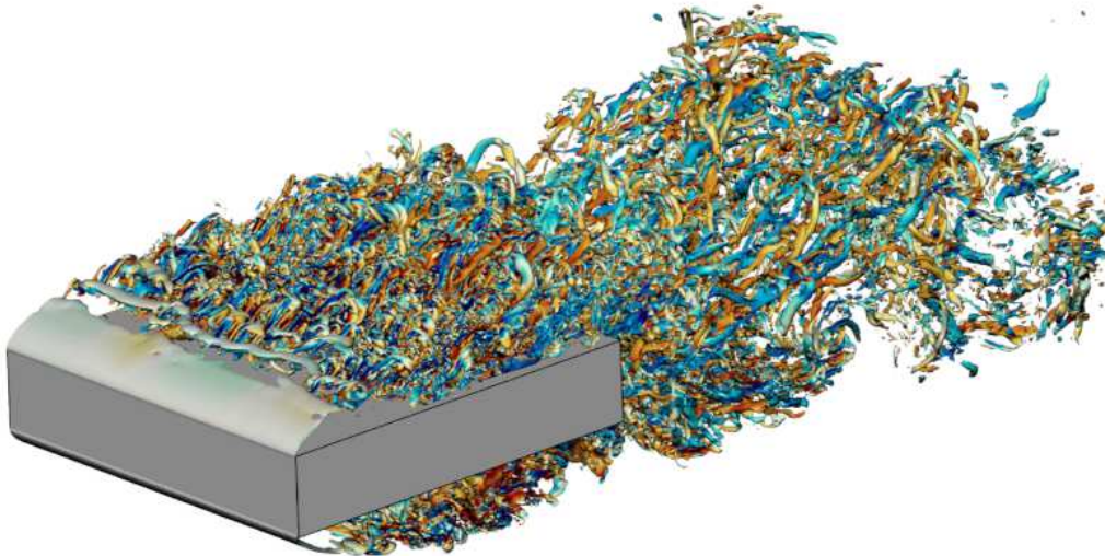
FIGURE 3. Instantaneous snapshot of the BARC flow: perspective view of the isosurfaces at \lambda_2 = -5 . Color depicts streamwise vorticity \omega_x , with the blue-to-red colormap ranging in -10 \leq \omega_x \leq 10 .
